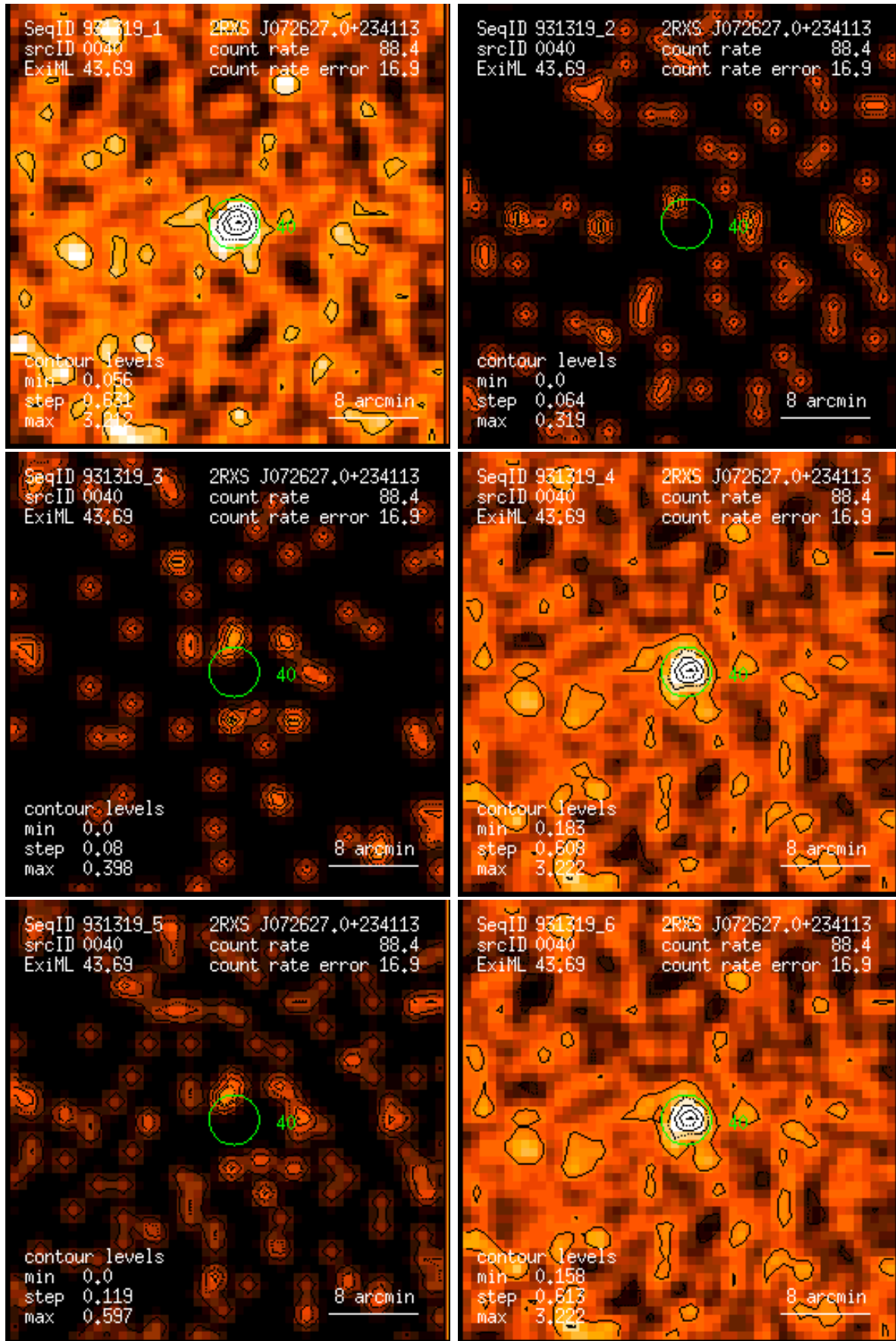
Figure 40: RASS 931319: detection 0040: band rate images, Gaussian filter: (1) PSPC channels 11 – 41, (2) 52 – 90, (3) 91 – 201, (4) 11 – 235, (5) 52 – 201, (6) 11 – 201. Broad band rates in counts/ks. Band rate contour levels in counts/ks/arcmin 2 .
