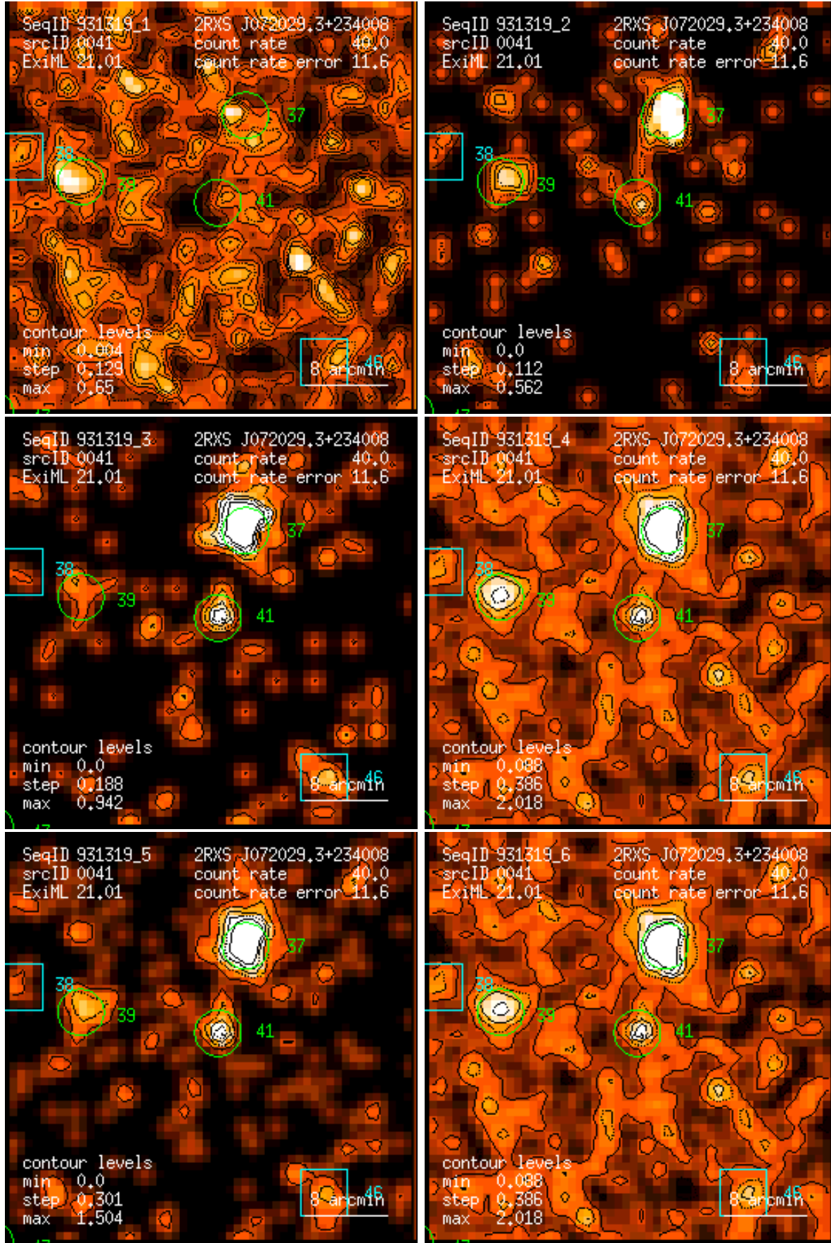
Figure 41: RASS 931319: detection 0041: band rate images, Gaussian filter: (1) PSPC channels 11 – 41, (2) 52 – 90, (3) 91 – 201, (4) 11 – 235, (5) 52 – 201, (6) 11 – 201. Broad band rates in counts/ks. Band rate contour levels in counts/ks/arcmin 2 .
