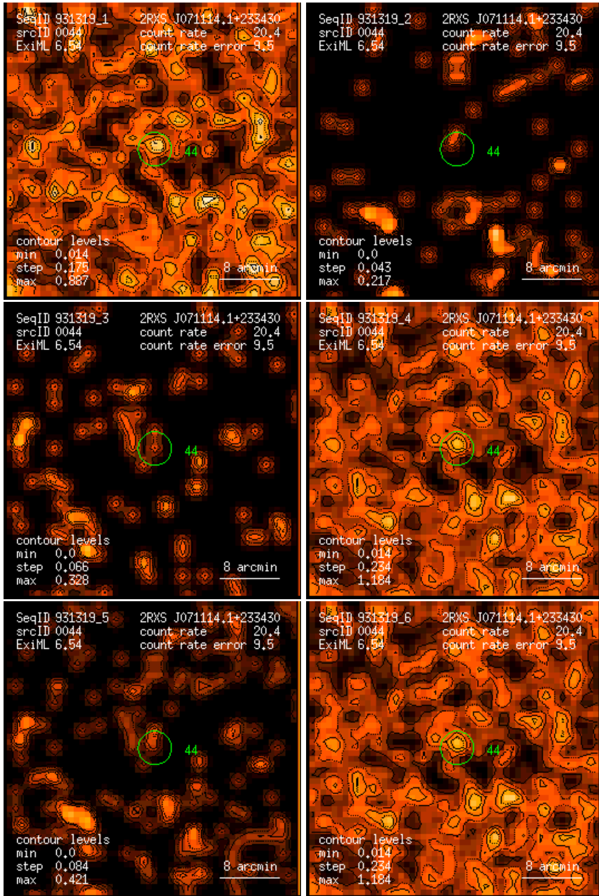
Figure 44: RASS 931319: detection 0044: band rate images, Gaussian filter: (1) PSPC channels 11 – 41, (2) 52 – 90, (3) 91 – 201, (4) 11 – 235, (5) 52 – 201, (6) 11 – 201. Broad band rates in counts/ks. Band rate contour levels in counts/ks/arcmin 2 .
