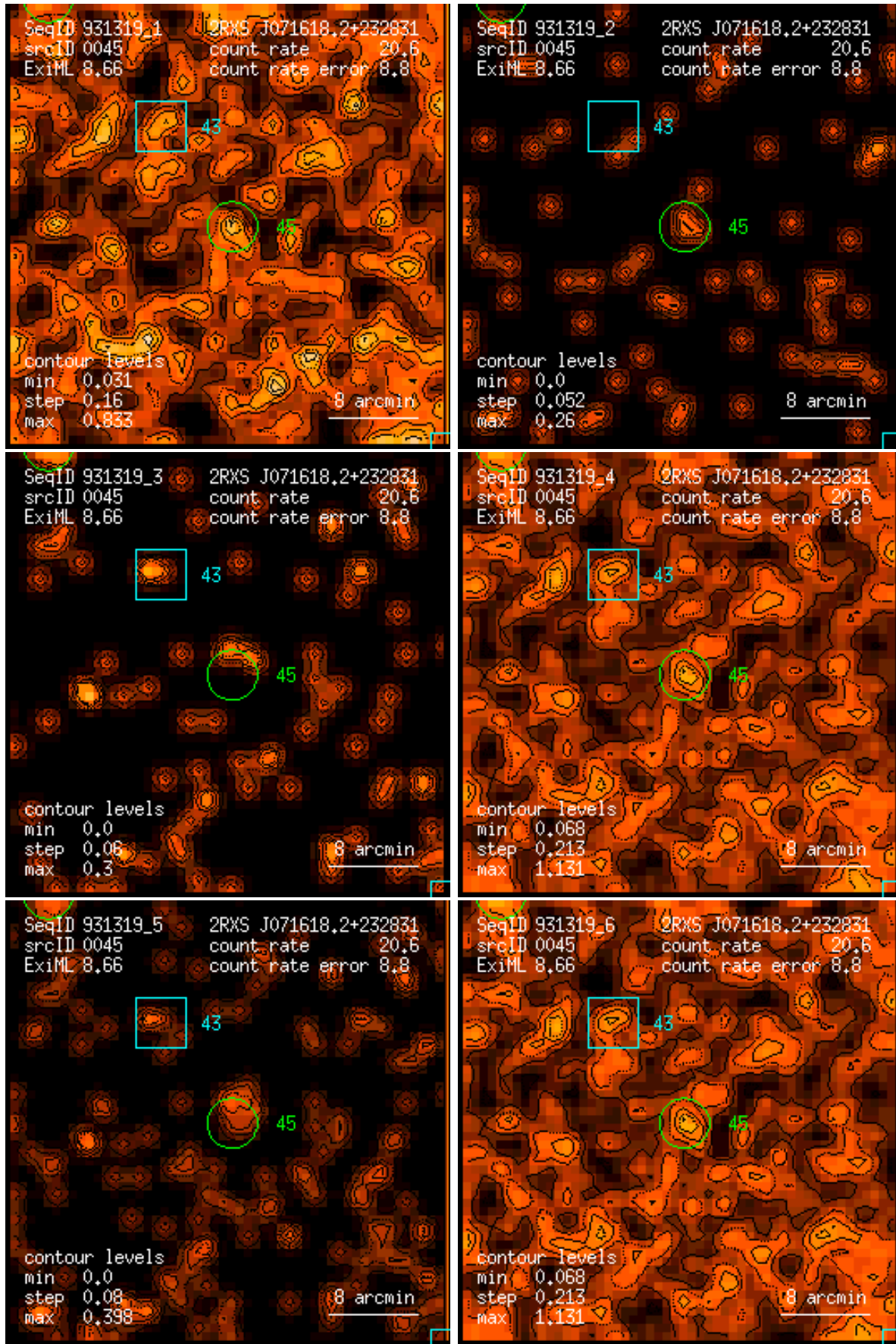
Figure 45: RASS 931319: detection 0045: band rate images, Gaussian filter: (1) PSPC channels 11 – 41, (2) 52 – 90, (3) 91 – 201, (4) 11 – 235, (5) 52 – 201, (6) 11 – 201. Broad band rates in counts/ks. Band rate contour levels in counts/ks/arcmin 2 .
