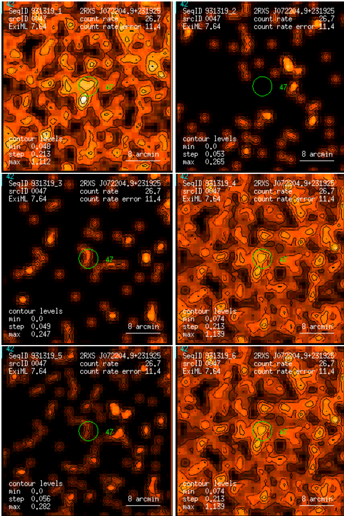
Figure 47: RASS 931319: detection 0047: band rate images, Gaussian filter: (1) PSPC channels 11 – 41, (2) 52 – 90, (3) 91 – 201, (4) 11 – 235, (5) 52 – 201, (6) 11 – 201. Broad band rates in counts/ks. Band rate contour levels in counts/ks/arcmin 2 .
