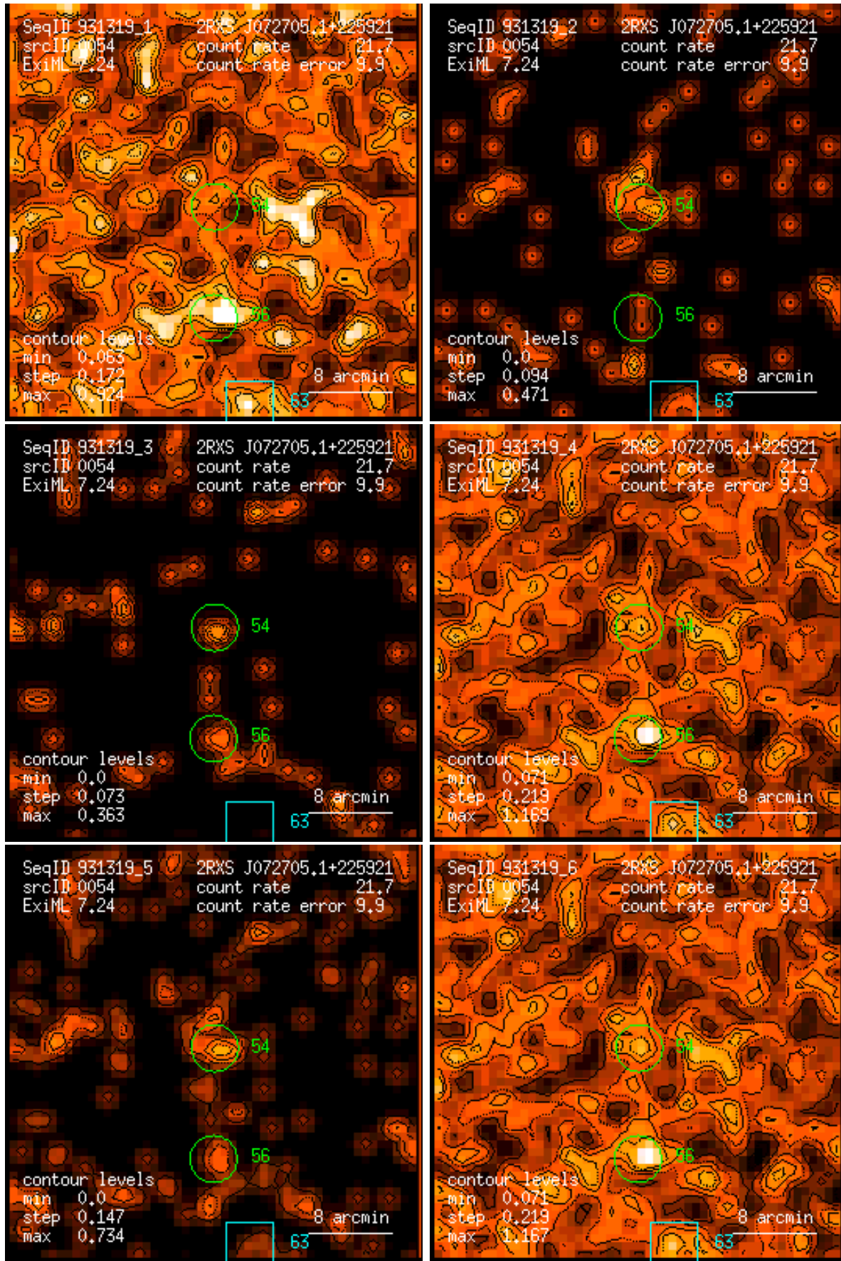
Figure 54: RASS 931319: detection 0054: band rate images, Gaussian filter: (1) PSPC channels 11 – 41, (2) 52 – 90, (3) 91 – 201, (4) 11 – 235, (5) 52 – 201, (6) 11 – 201. Broad band rates in counts/ks. Band rate contour levels in counts/ks/arcmin 2 .
