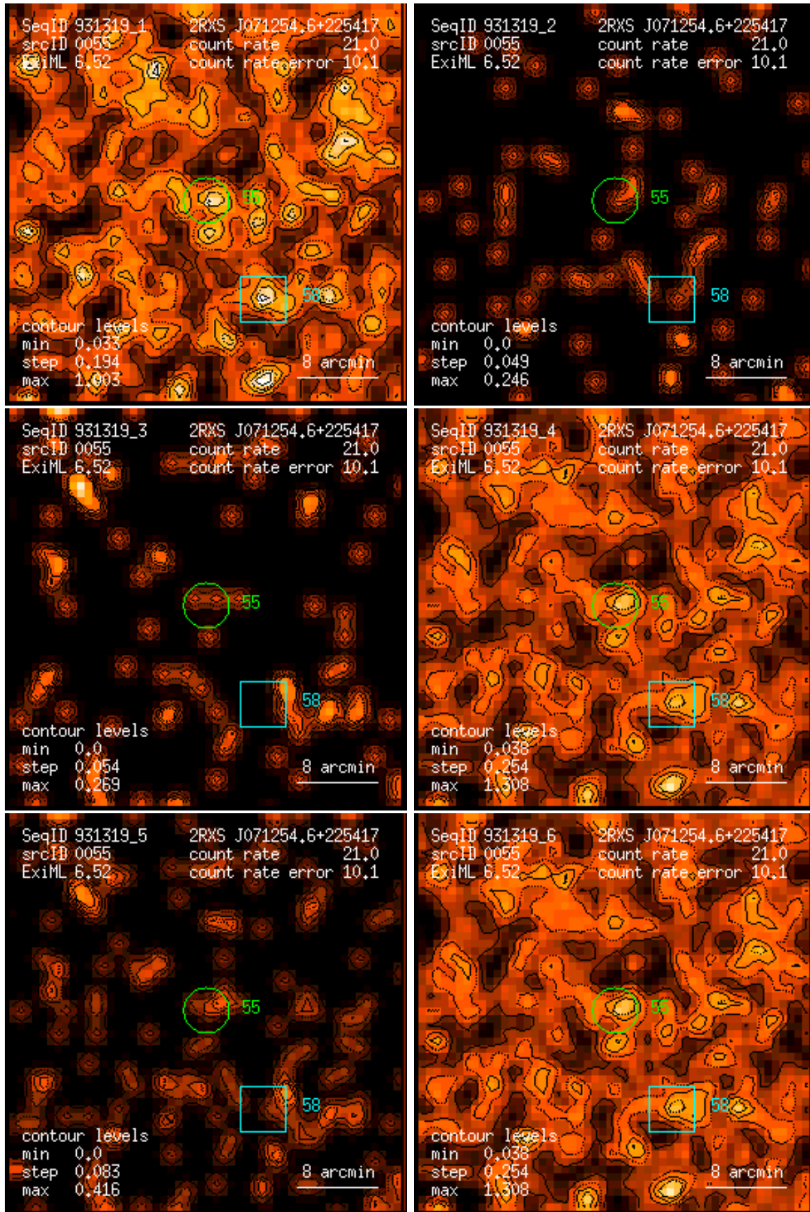
Figure 55: RASS 931319: detection 0055: band rate images, Gaussian filter: (1) PSPC channels 11 – 41, (2) 52 – 90, (3) 91 – 201, (4) 11 – 235, (5) 52 – 201, (6) 11 – 201. Broad band rates in counts/ks. Band rate contour levels in counts/ks/arcmin 2 .
