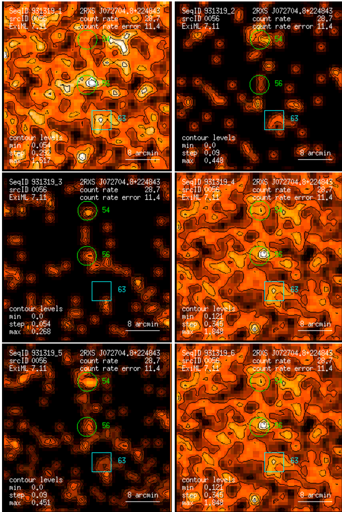
Figure 56: RASS 931319: detection 0056: band rate images, Gaussian filter: (1) PSPC channels 11 – 41, (2) 52 – 90, (3) 91 – 201, (4) 11 – 235, (5) 52 – 201, (6) 11 – 201. Broad band rates in counts/ks. Band rate contour levels in counts/ks/arcmin 2 .
