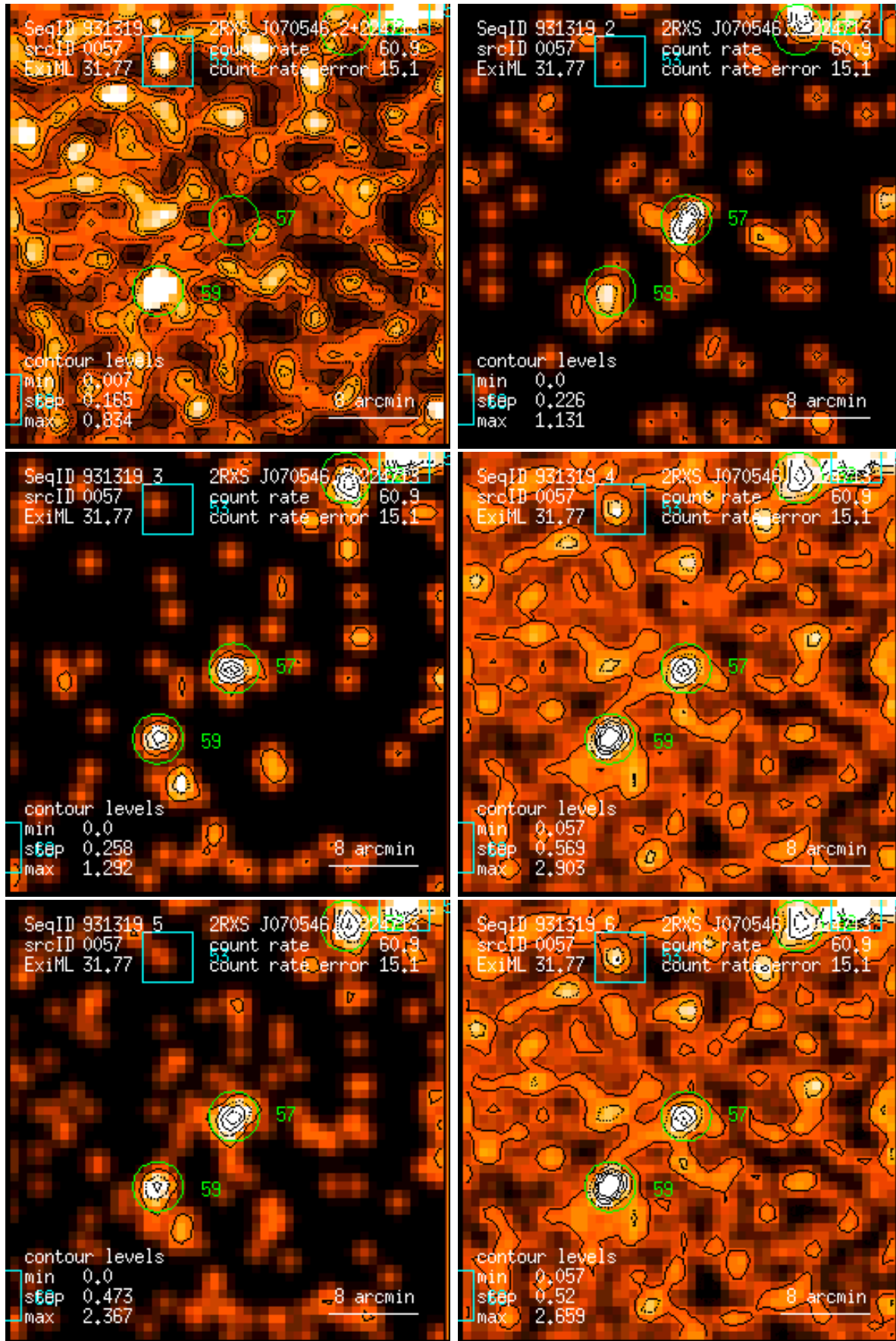
Figure 57: RASS 931319: detection 0057: band rate images, Gaussian filter: (1) PSPC channels 11 – 41, (2) 52 – 90, (3) 91 – 201, (4) 11 – 235, (5) 52 – 201, (6) 11 – 201. Broad band rates in counts/ks. Band rate contour levels in counts/ks/arcmin 2 .
