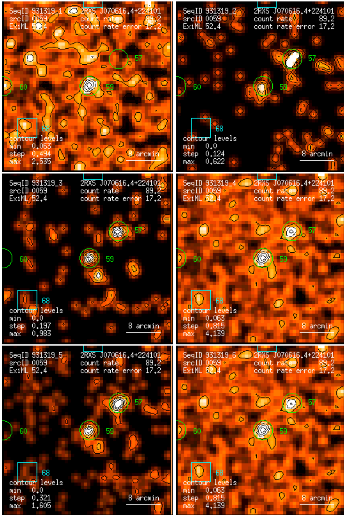
Figure 59: RASS 931319: detection 0059: band rate images, Gaussian filter: (1) PSPC channels 11 – 41, (2) 52 – 90, (3) 91 – 201, (4) 11 – 235, (5) 52 – 201, (6) 11 – 201. Broad band rates in counts/ks. Band rate contour levels in counts/ks/arcmin 2 .
