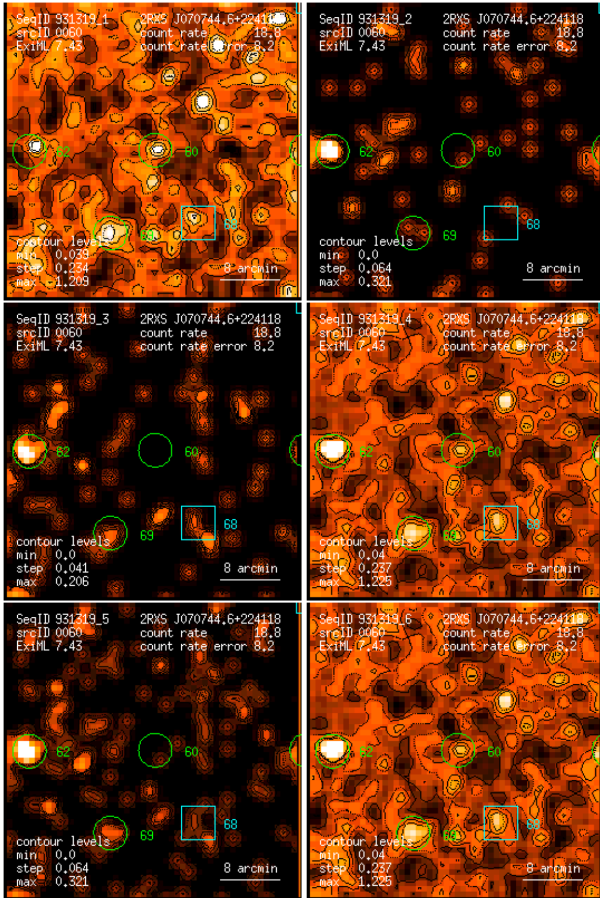
Figure 60: RASS 931319: detection 0060: band rate images, Gaussian filter: (1) PSPC channels 11 – 41, (2) 52 – 90, (3) 91 – 201, (4) 11 – 235, (5) 52 – 201, (6) 11 – 201. Broad band rates in counts/ks. Band rate contour levels in counts/ks/arcmin 2 .
