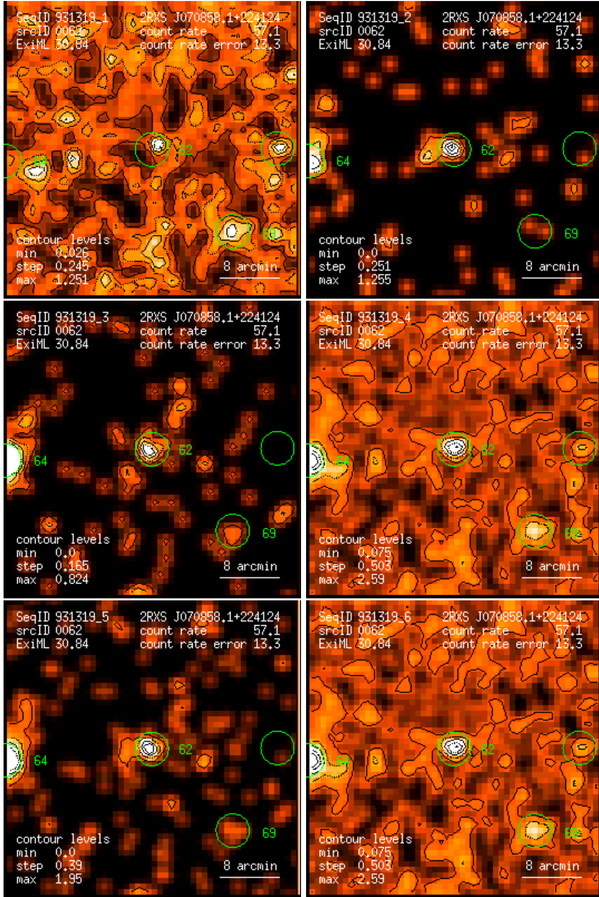
Figure 62: RASS 931319: detection 0062: band rate images, Gaussian filter: (1) PSPC channels 11 – 41, (2) 52 – 90, (3) 91 – 201, (4) 11 – 235, (5) 52 – 201, (6) 11 – 201. Broad band rates in counts/ks. Band rate contour levels in counts/ks/arcmin 2 .
