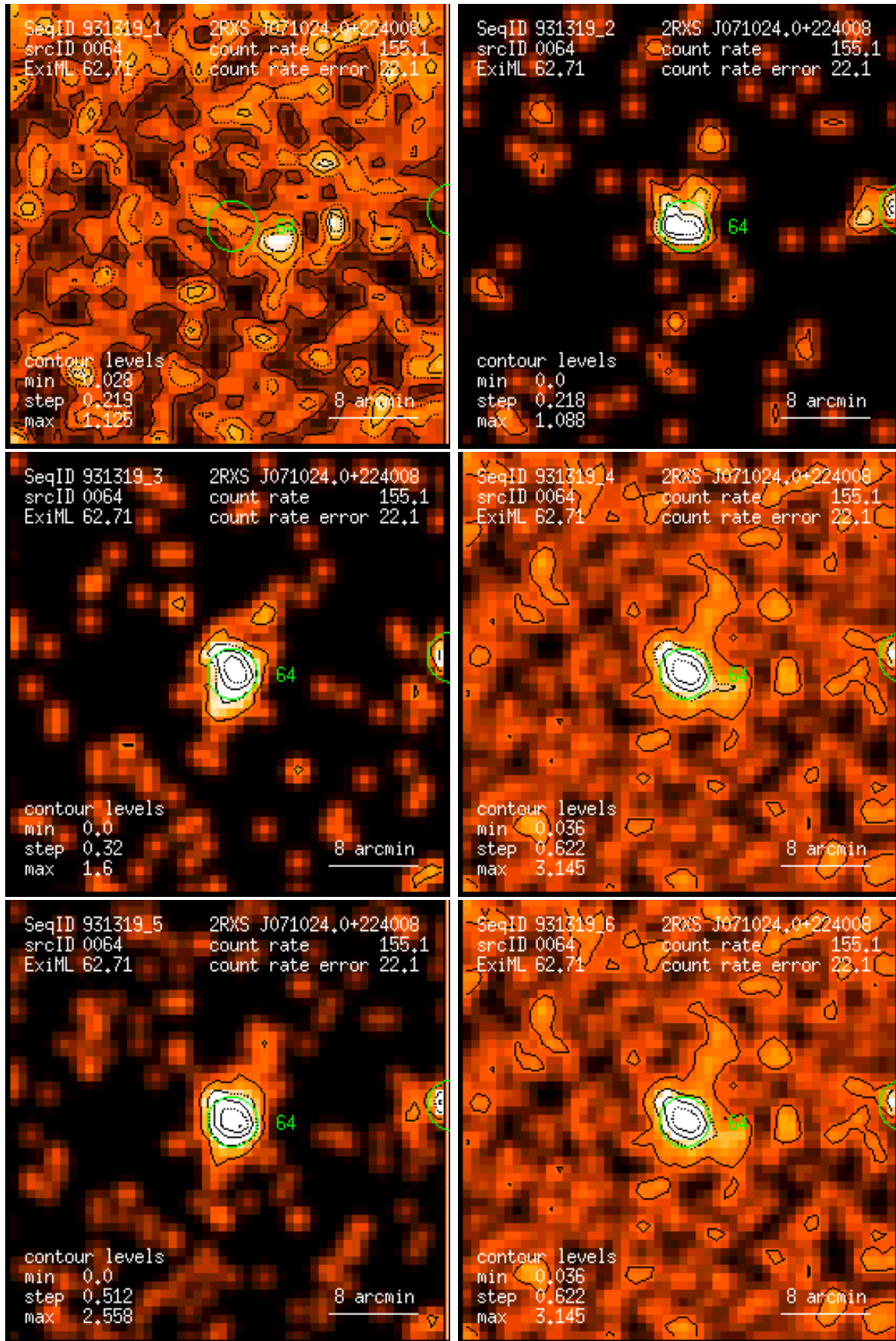
Figure 64: RASS 931319: detection 0064: band rate images, Gaussian filter: (1) PSPC channels 11 – 41, (2) 52 – 90, (3) 91 – 201, (4) 11 – 235, (5) 52 – 201, (6) 11 – 201. Broad band rates in counts/ks. Band rate contour levels in counts/ks/arcmin 2 .
