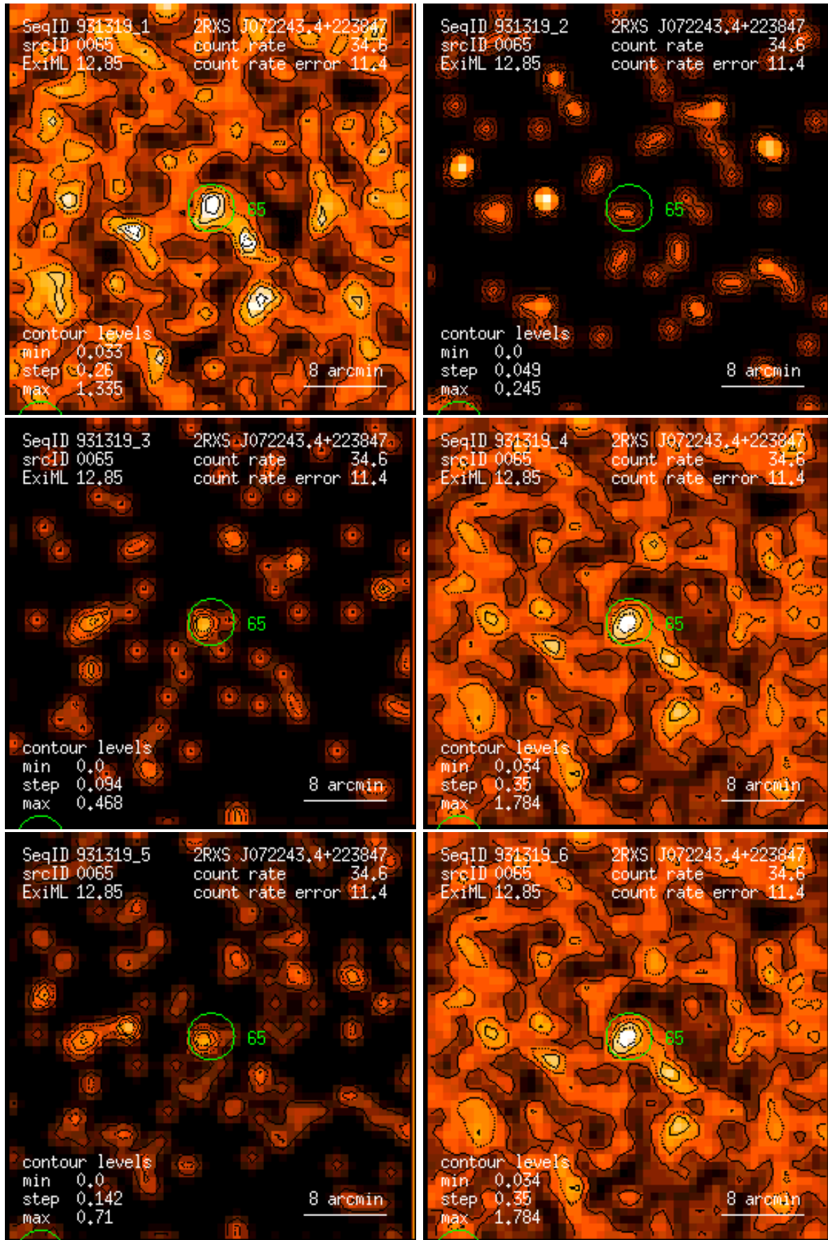
Figure 65: RASS 931319: detection 0065: band rate images, Gaussian filter: (1) PSPC channels 11 – 41, (2) 52 – 90, (3) 91 – 201, (4) 11 – 235, (5) 52 – 201, (6) 11 – 201. Broad band rates in counts/ks. Band rate contour levels in counts/ks/arcmin 2 .
