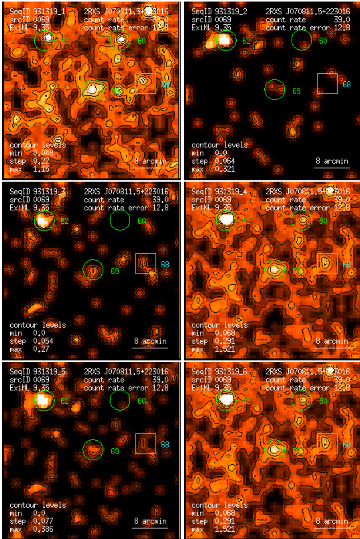
Figure 69: RASS 931319: detection 0069: band rate images, Gaussian filter: (1) PSPC channels 11 – 41, (2) 52 – 90, (3) 91 – 201, (4) 11 – 235, (5) 52 – 201, (6) 11 – 201. Broad band rates in counts/ks. Band rate contour levels in counts/ks/arcmin 2 .
