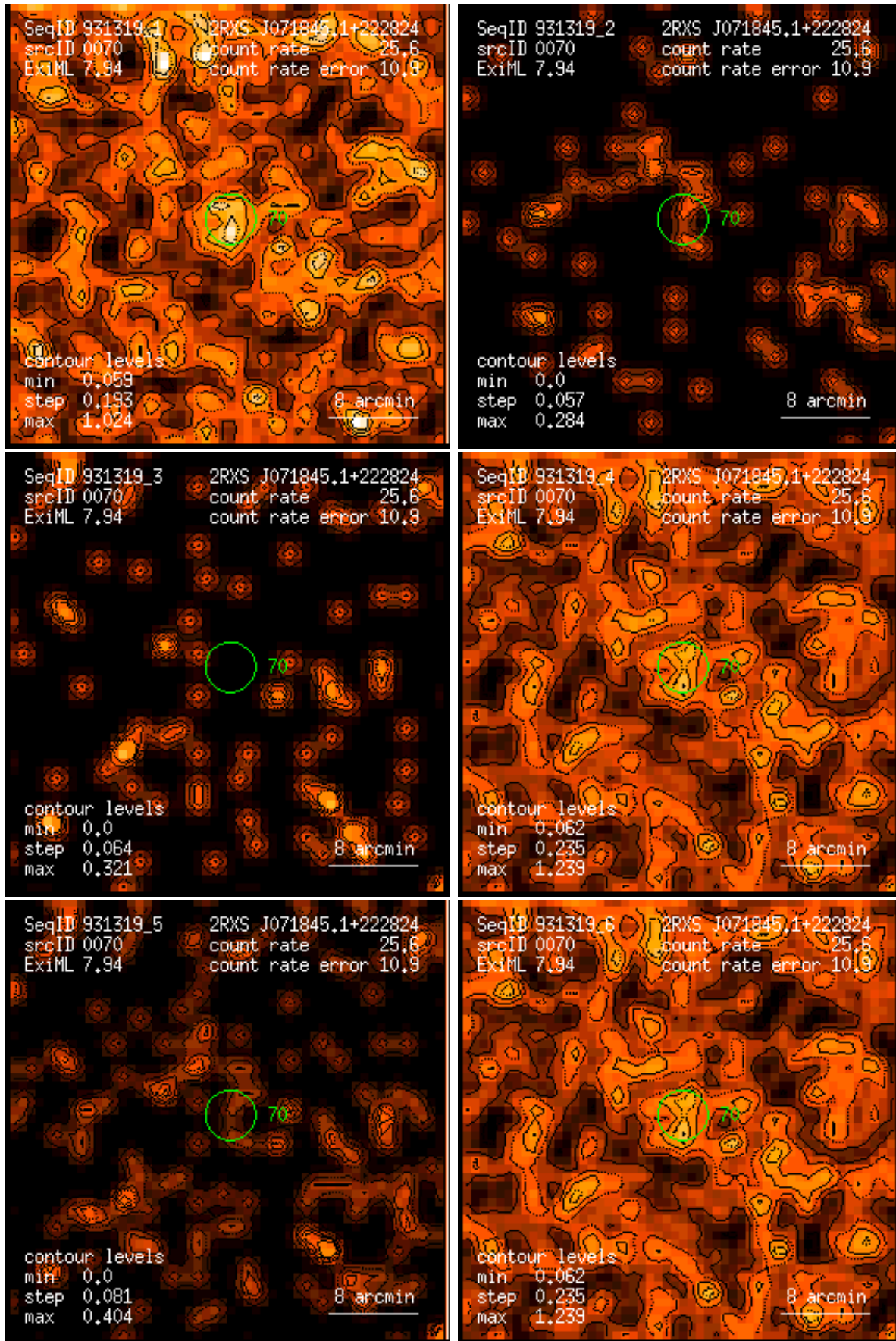
Figure 70: RASS 931319: detection 0070: band rate images, Gaussian filter: (1) PSPC channels 11 – 41, (2) 52 – 90, (3) 91 – 201, (4) 11 – 235, (5) 52 – 201, (6) 11 – 201. Broad band rates in counts/ks. Band rate contour levels in counts/ks/arcmin 2 .
