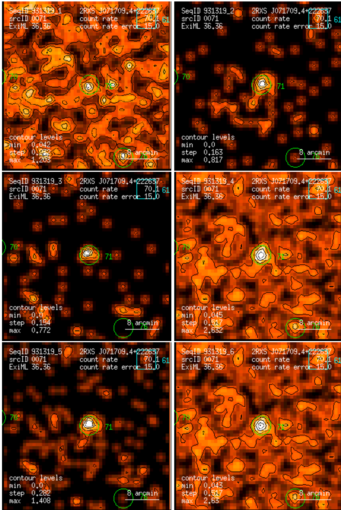
Figure 71: RASS 931319: detection 0071: band rate images, Gaussian filter: (1) PSPC channels 11 – 41, (2) 52 – 90, (3) 91 – 201, (4) 11 – 235, (5) 52 – 201, (6) 11 – 201. Broad band rates in counts/ks. Band rate contour levels in counts/ks/arcmin 2 .
