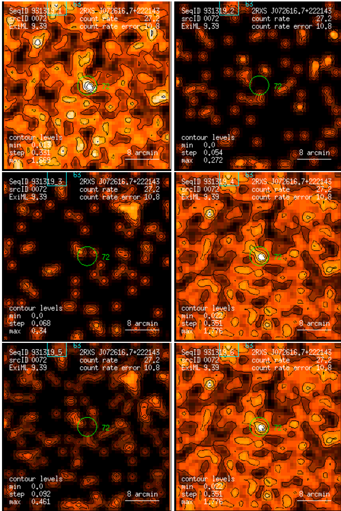
Figure 72: RASS 931319: detection 0072: band rate images, Gaussian filter: (1) PSPC channels 11 – 41, (2) 52 – 90, (3) 91 – 201, (4) 11 – 235, (5) 52 – 201, (6) 11 – 201. Broad band rates in counts/ks. Band rate contour levels in counts/ks/arcmin 2 .
