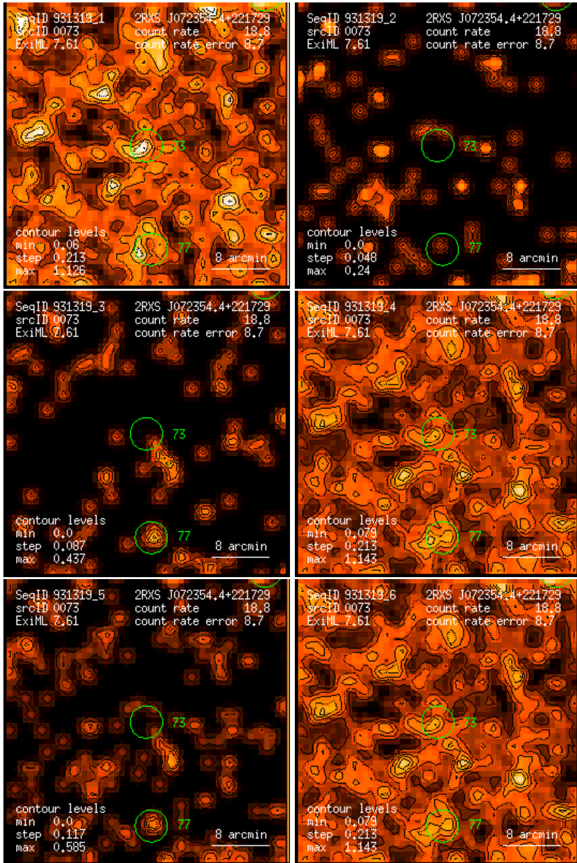
Figure 73: RASS 931319: detection 0073: band rate images, Gaussian filter: (1) PSPC channels 11 – 41, (2) 52 – 90, (3) 91 – 201, (4) 11 – 235, (5) 52 – 201, (6) 11 – 201. Broad band rates in counts/ks. Band rate contour levels in counts/ks/arcmin 2 .
