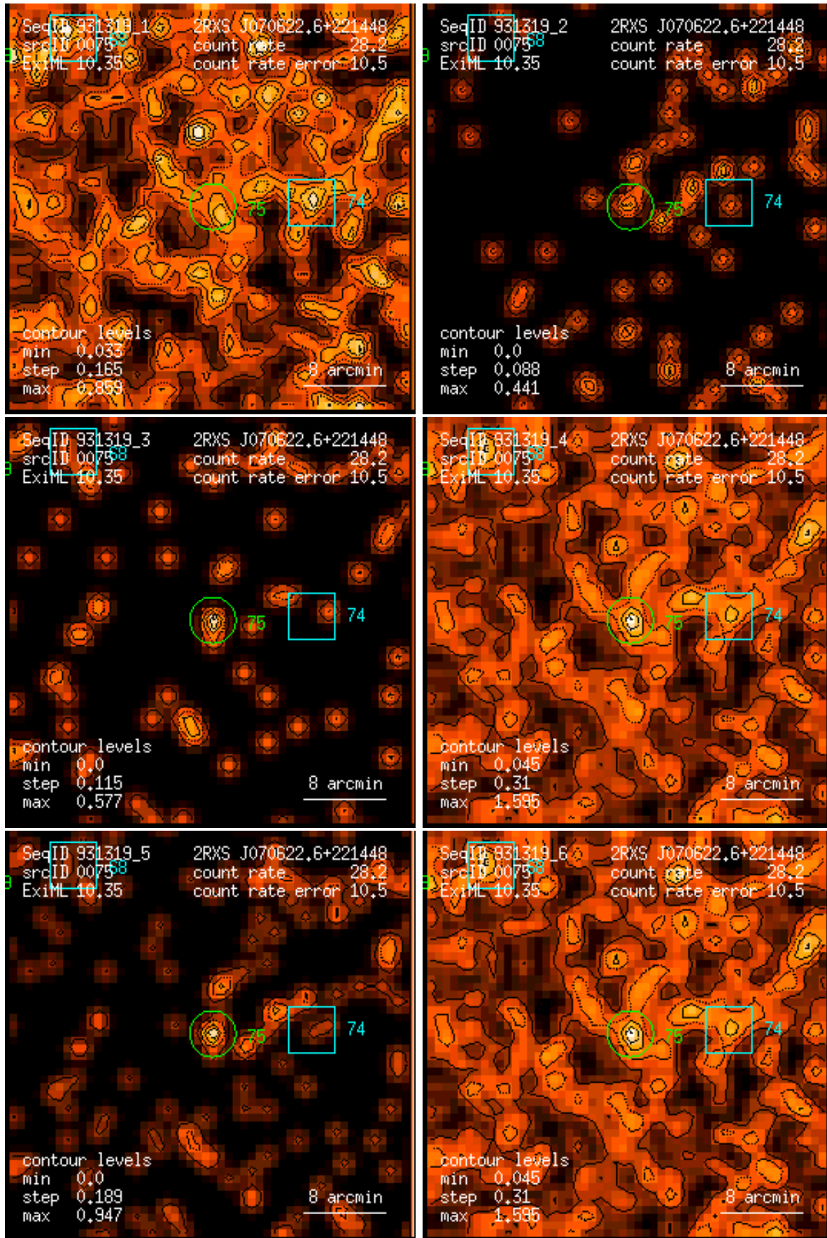
Figure 75: RASS 931319: detection 0075: band rate images, Gaussian filter: (1) PSPC channels 11 – 41, (2) 52 – 90, (3) 91 – 201, (4) 11 – 235, (5) 52 – 201, (6) 11 – 201. Broad band rates in counts/ks. Band rate contour levels in counts/ks/arcmin 2 .
