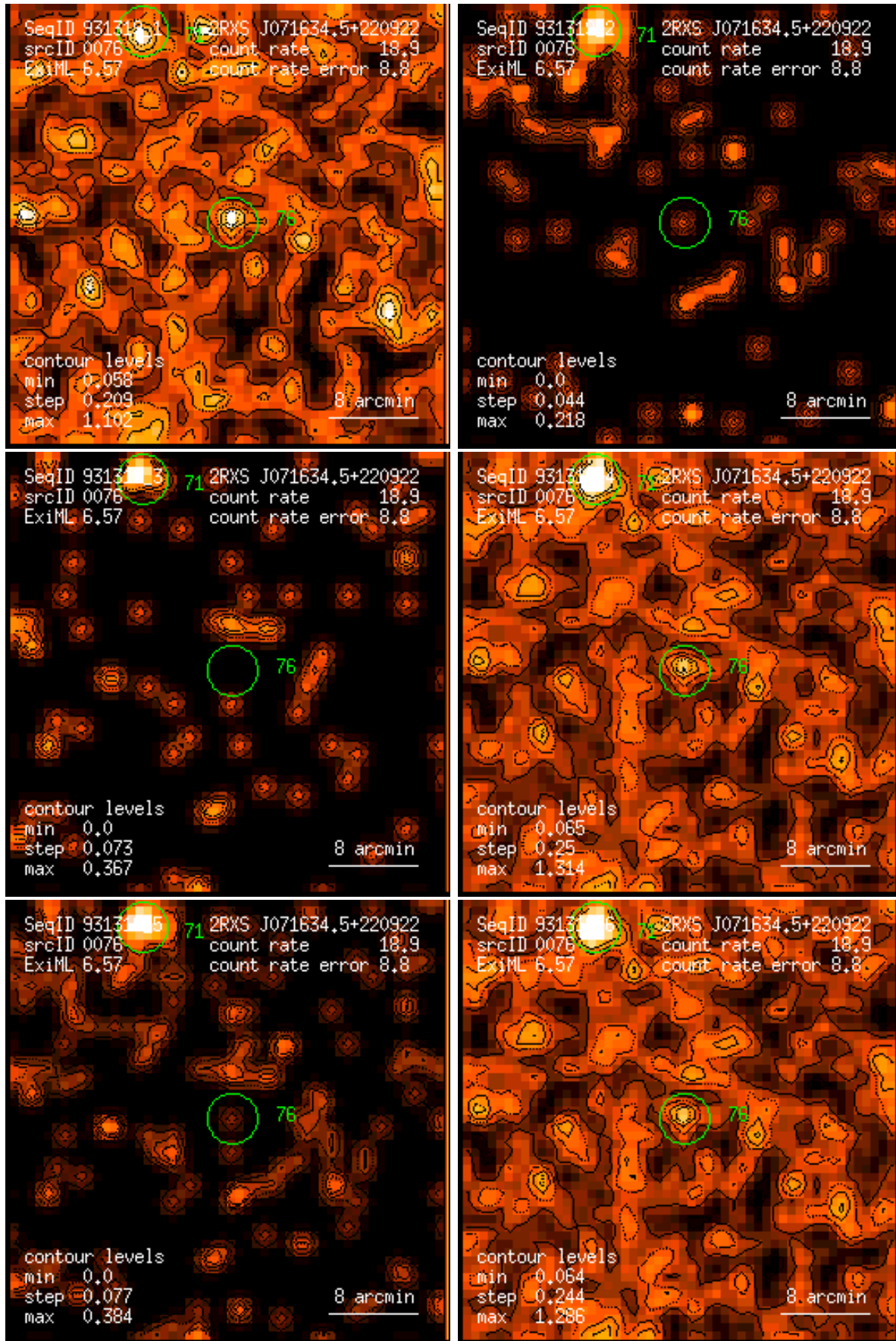
Figure 76: RASS 931319: detection 0076: band rate images, Gaussian filter: (1) PSPC channels 11 – 41, (2) 52 – 90, (3) 91 – 201, (4) 11 – 235, (5) 52 – 201, (6) 11 – 201. Broad band rates in counts/ks. Band rate contour levels in counts/ks/arcmin 2 .
