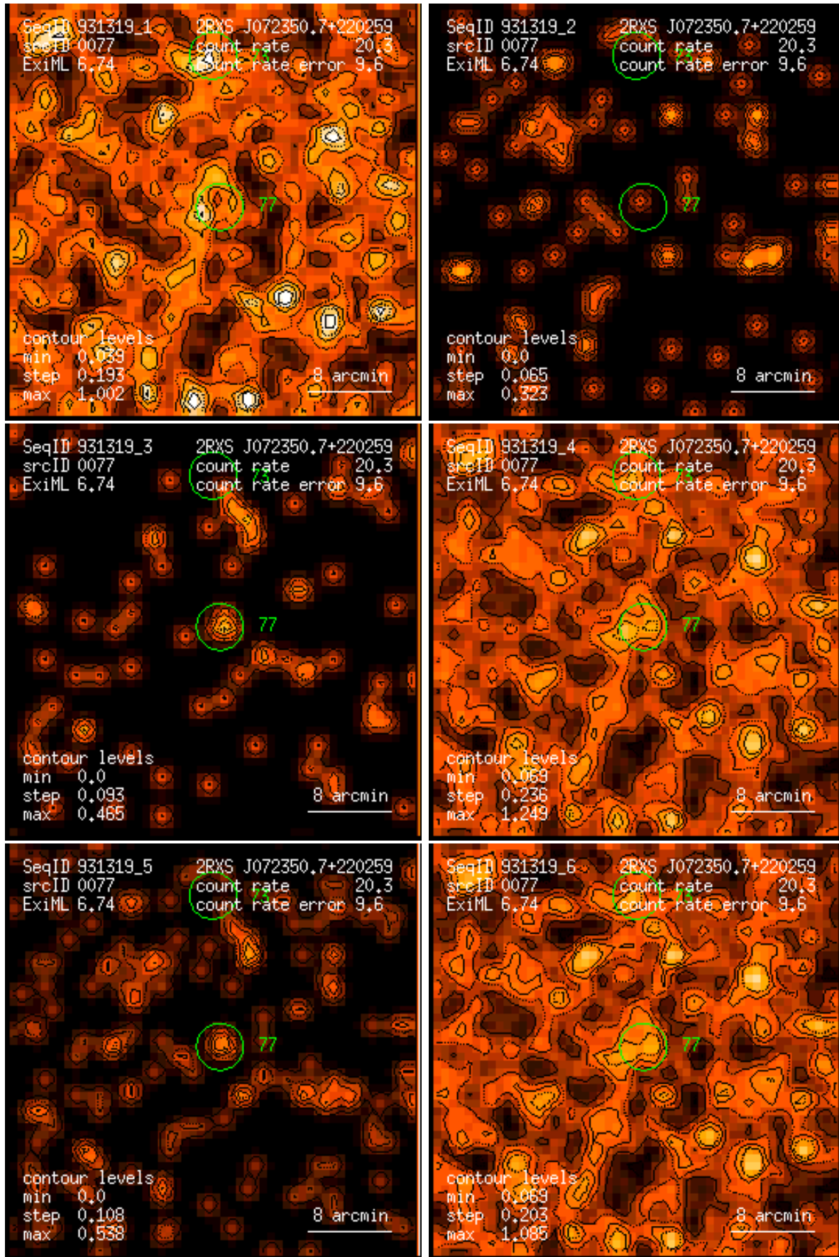
Figure 77: RASS 931319: detection 0077: band rate images, Gaussian filter: (1) PSPC channels 11 – 41, (2) 52 – 90, (3) 91 – 201, (4) 11 – 235, (5) 52 – 201, (6) 11 – 201. Broad band rates in counts/ks. Band rate contour levels in counts/ks/arcmin 2 .
