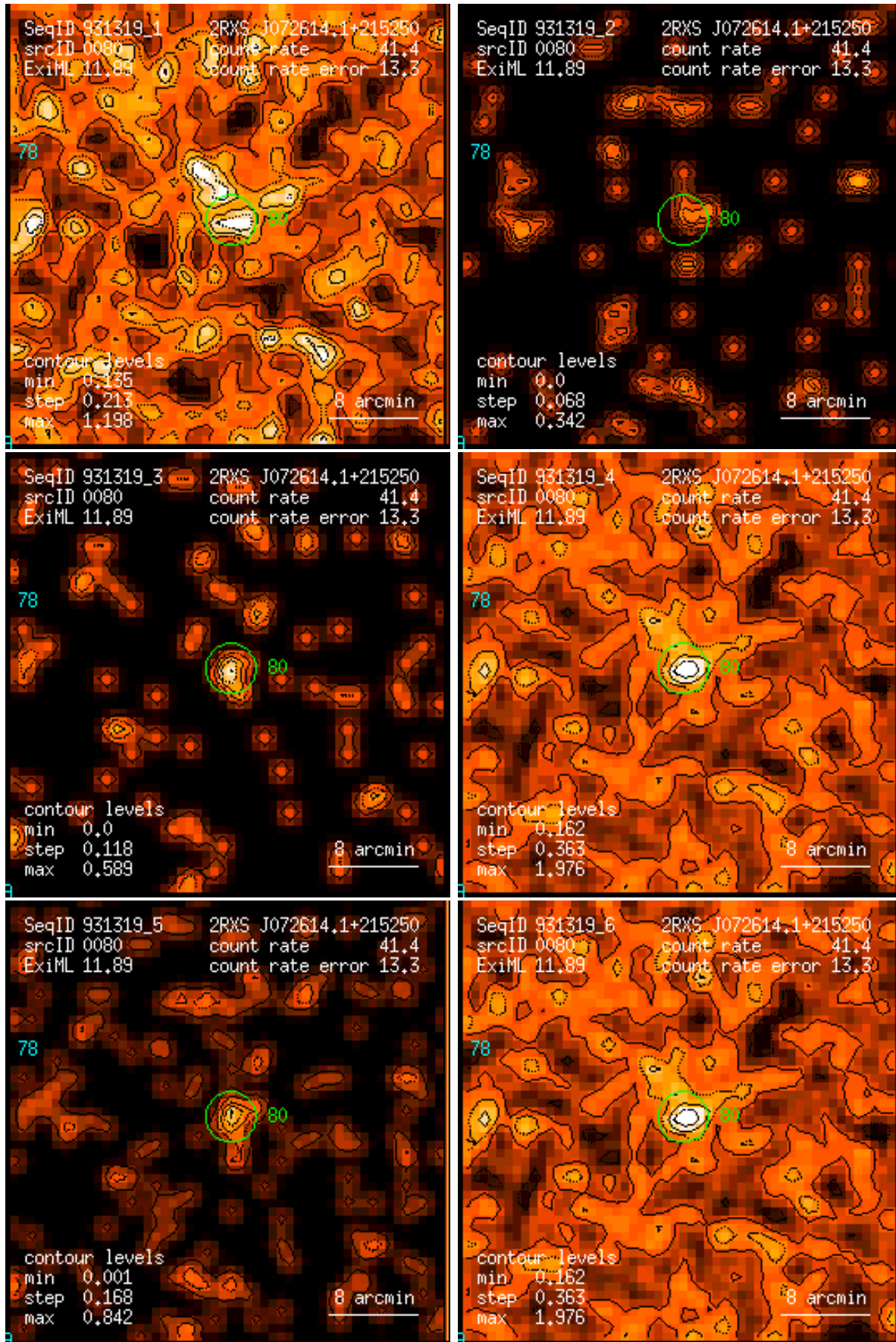
Figure 80: RASS 931319: detection 0080: band rate images, Gaussian filter: (1) PSPC channels 11 – 41, (2) 52 – 90, (3) 91 – 201, (4) 11 – 235, (5) 52 – 201, (6) 11 – 201. Broad band rates in counts/ks. Band rate contour levels in counts/ks/arcmin 2 .
