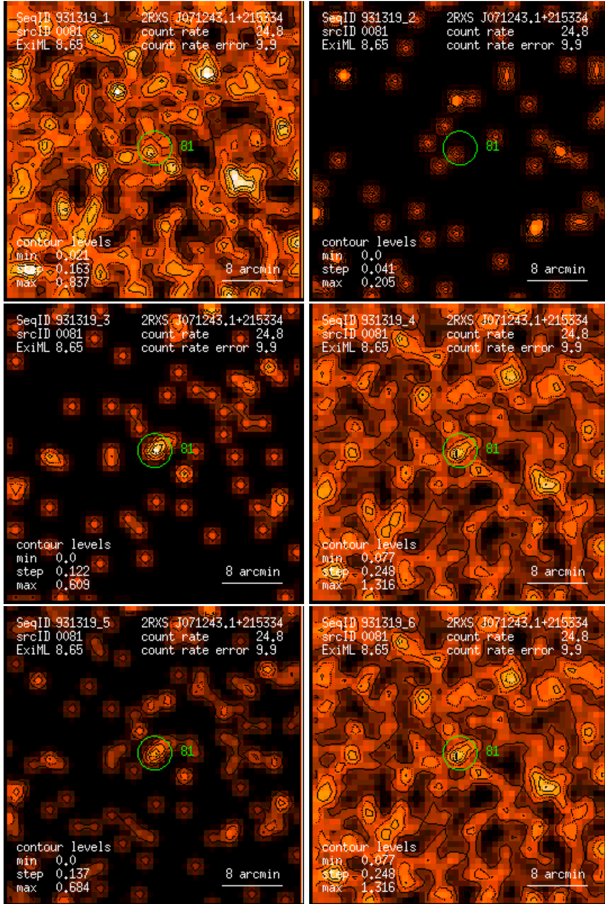
Figure 81: RASS 931319: detection 0081: band rate images, Gaussian filter: (1) PSPC channels 11 – 41, (2) 52 – 90, (3) 91 – 201, (4) 11 – 235, (5) 52 – 201, (6) 11 – 201. Broad band rates in counts/ks. Band rate contour levels in counts/ks/arcmin 2 .
