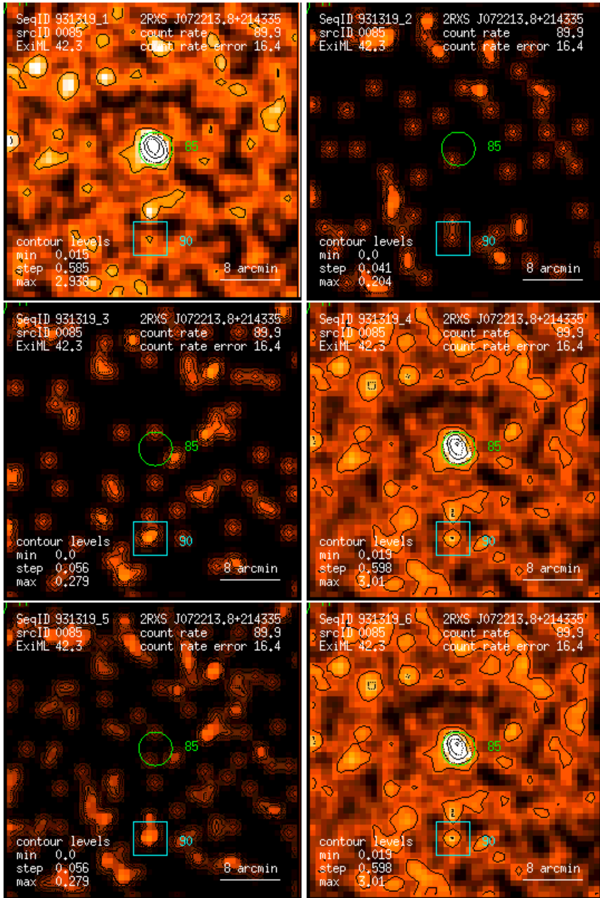
Figure 85: RASS 931319: detection 0085: band rate images, Gaussian filter: (1) PSPC channels 11 – 41, (2) 52 – 90, (3) 91 – 201, (4) 11 – 235, (5) 52 – 201, (6) 11 – 201. Broad band rates in counts/ks. Band rate contour levels in counts/ks/arcmin 2 .
