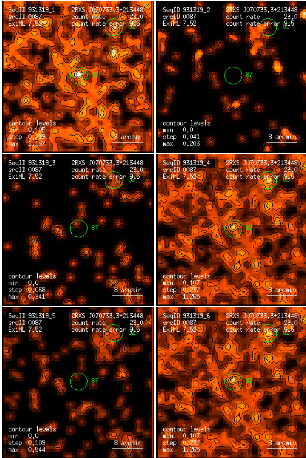
Figure 87: RASS 931319: detection 0087: band rate images, Gaussian filter: (1) PSPC channels 11 – 41, (2) 52 – 90, (3) 91 – 201, (4) 11 – 235, (5) 52 – 201, (6) 11 – 201. Broad band rates in counts/ks. Band rate contour levels in counts/ks/arcmin 2 .
