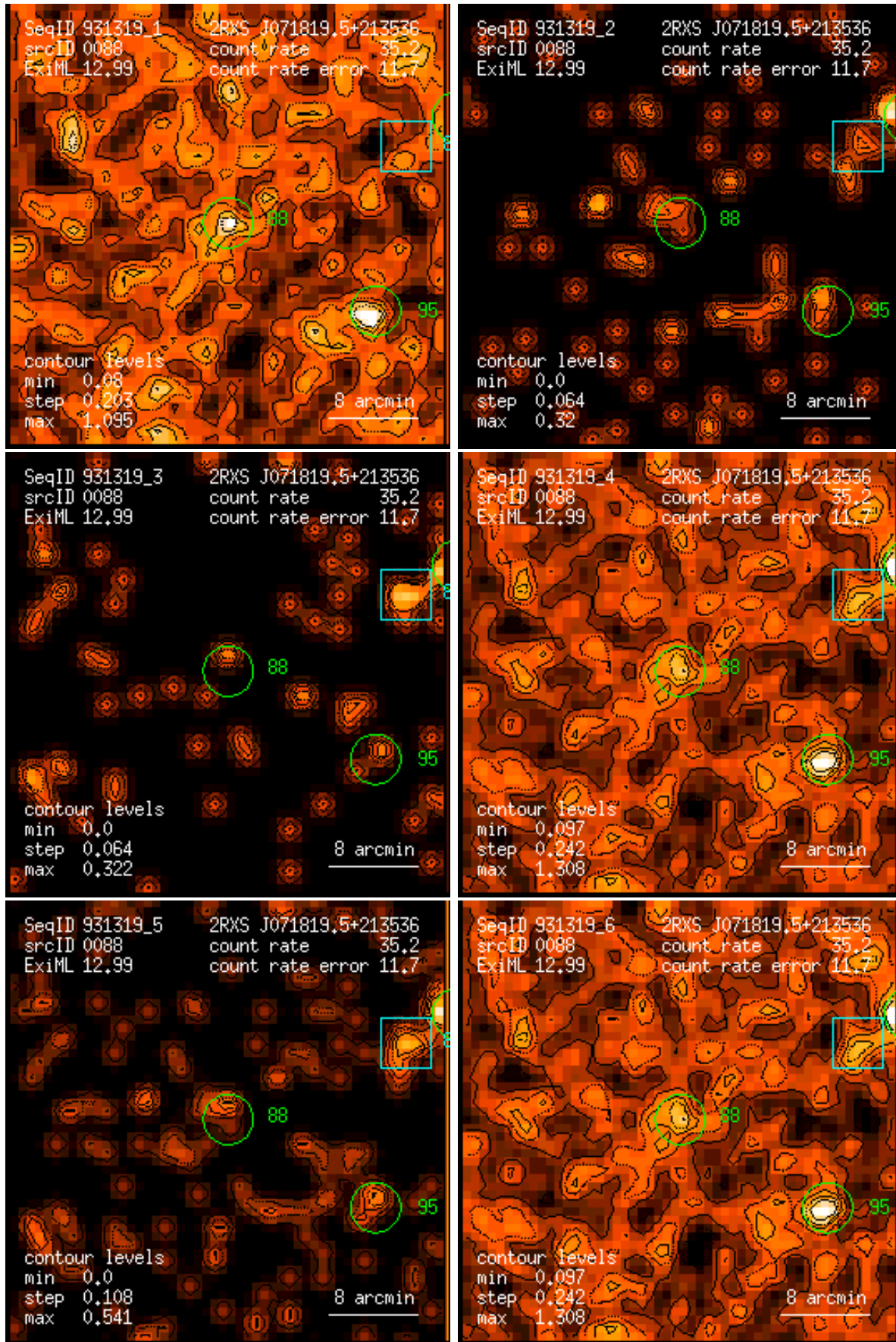
Figure 88: RASS 931319: detection 0088: band rate images, Gaussian filter: (1) PSPC channels 11 – 41, (2) 52 – 90, (3) 91 – 201, (4) 11 – 235, (5) 52 – 201, (6) 11 – 201. Broad band rates in counts/ks. Band rate contour levels in counts/ks/arcmin 2 .
