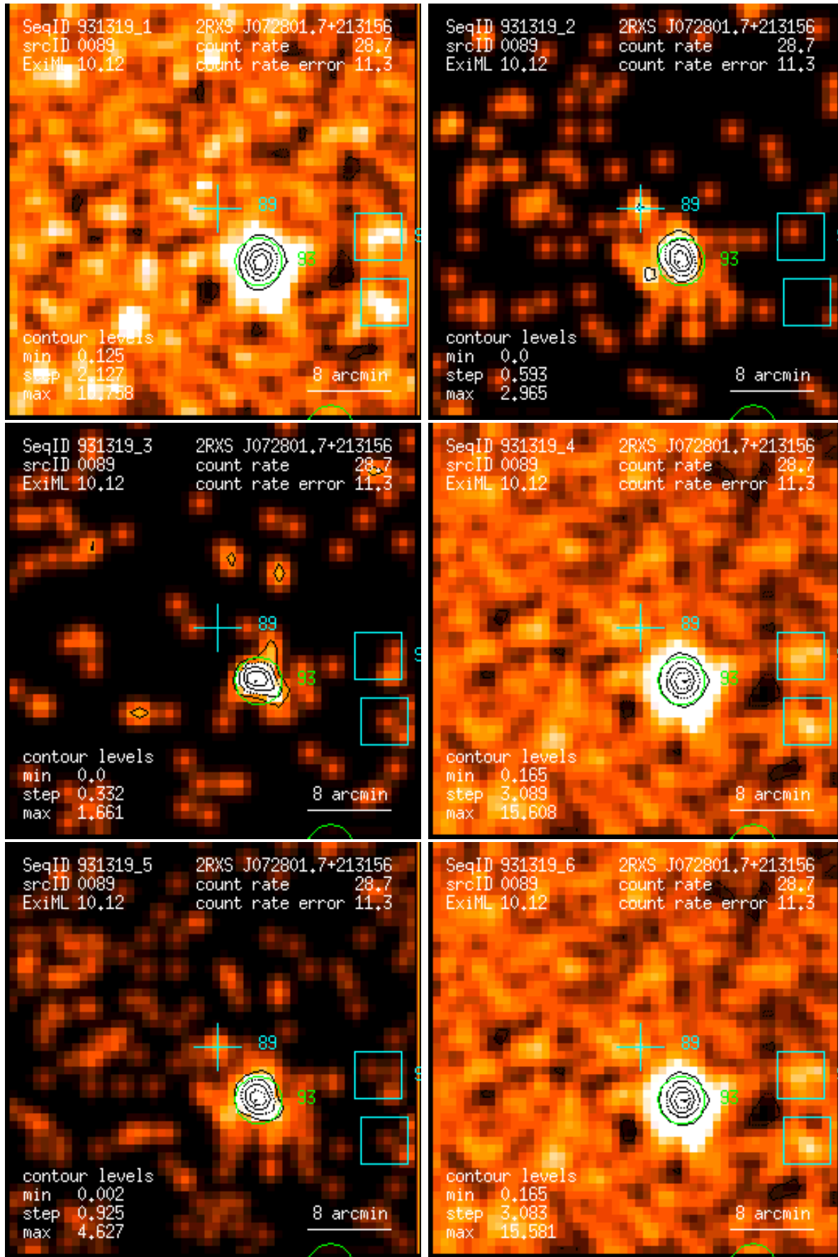
Figure 89: RASS 931319: detection 0089: band rate images, Gaussian filter: (1) PSPC channels 11 – 41, (2) 52 – 90, (3) 91 – 201, (4) 11 – 235, (5) 52 – 201, (6) 11 – 201. Broad band rates in counts/ks. Band rate contour levels in counts/ks/arcmin 2 .
