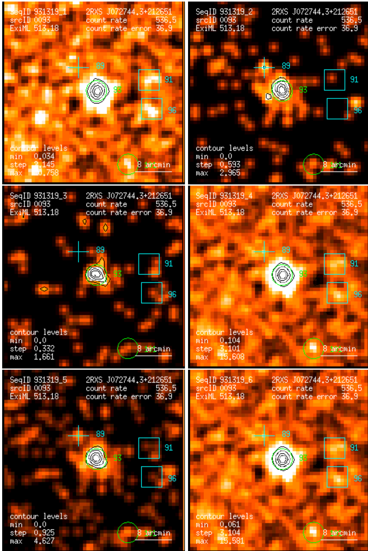
Figure 93: RASS 931319: detection 0093: band rate images, Gaussian filter: (1) PSPC channels 11 – 41, (2) 52 – 90, (3) 91 – 201, (4) 11 – 235, (5) 52 – 201, (6) 11 – 201. Broad band rates in counts/ks. Band rate contour levels in counts/ks/arcmin 2 .
