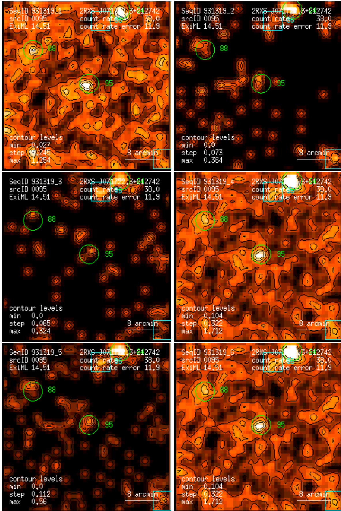
Figure 95: RASS 931319: detection 0095: band rate images, Gaussian filter: (1) PSPC channels 11 – 41, (2) 52 – 90, (3) 91 – 201, (4) 11 – 235, (5) 52 – 201, (6) 11 – 201. Broad band rates in counts/ks. Band rate contour levels in counts/ks/arcmin 2 .
