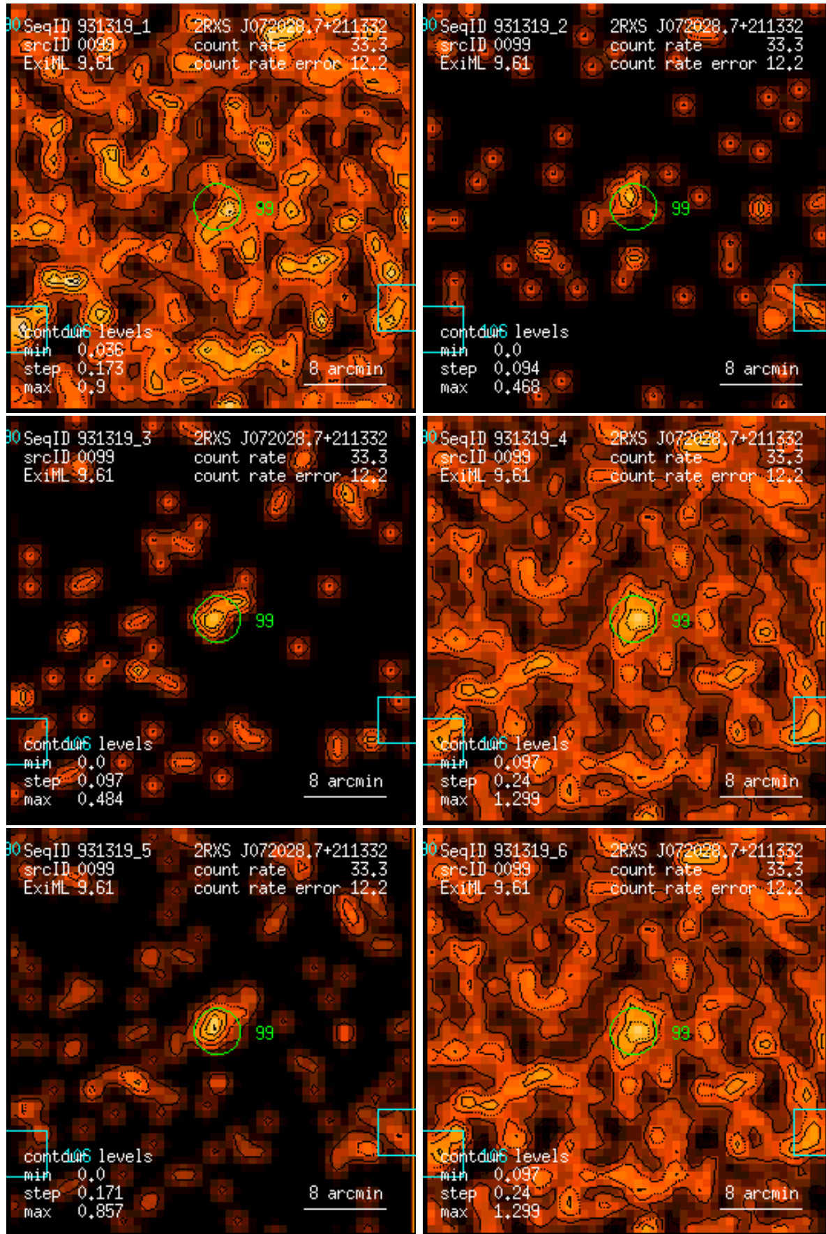
Figure 99: RASS 931319: detection 0099: band rate images, Gaussian filter: (1) PSPC channels 11 – 41, (2) 52 – 90, (3) 91 – 201, (4) 11 – 235, (5) 52 – 201, (6) 11 – 201. Broad band rates in counts/ks. Band rate contour levels in counts/ks/arcmin 2 .
