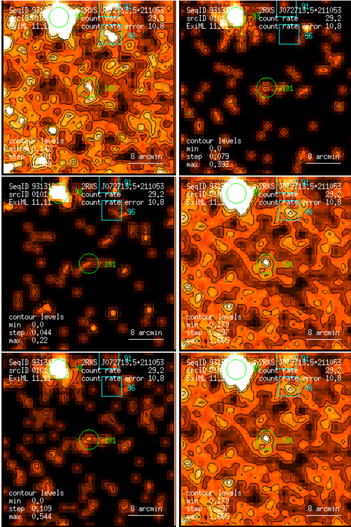
Figure 101: RASS 931319: detection 0101: band rate images, Gaussian filter: (1) PSPC channels 11 – 41, (2) 52 – 90, (3) 91 – 201, (4) 11 – 235, (5) 52 – 201, (6) 11 – 201. Broad band rates in counts/ks. Band rate contour levels in counts/ks/arcmin 2 .
