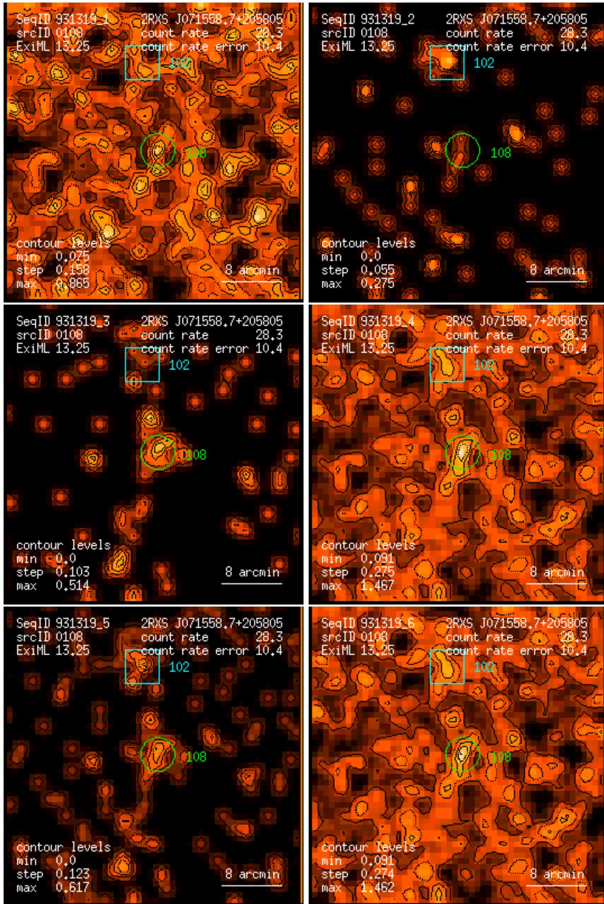
Figure 108: RASS 931319: detection 0108: band rate images, Gaussian filter: (1) PSPC channels 11 – 41, (2) 52 – 90, (3) 91 – 201, (4) 11 – 235, (5) 52 – 201, (6) 11 – 201. Broad band rates in counts/ks. Band rate contour levels in counts/ks/arcmin 2 .
