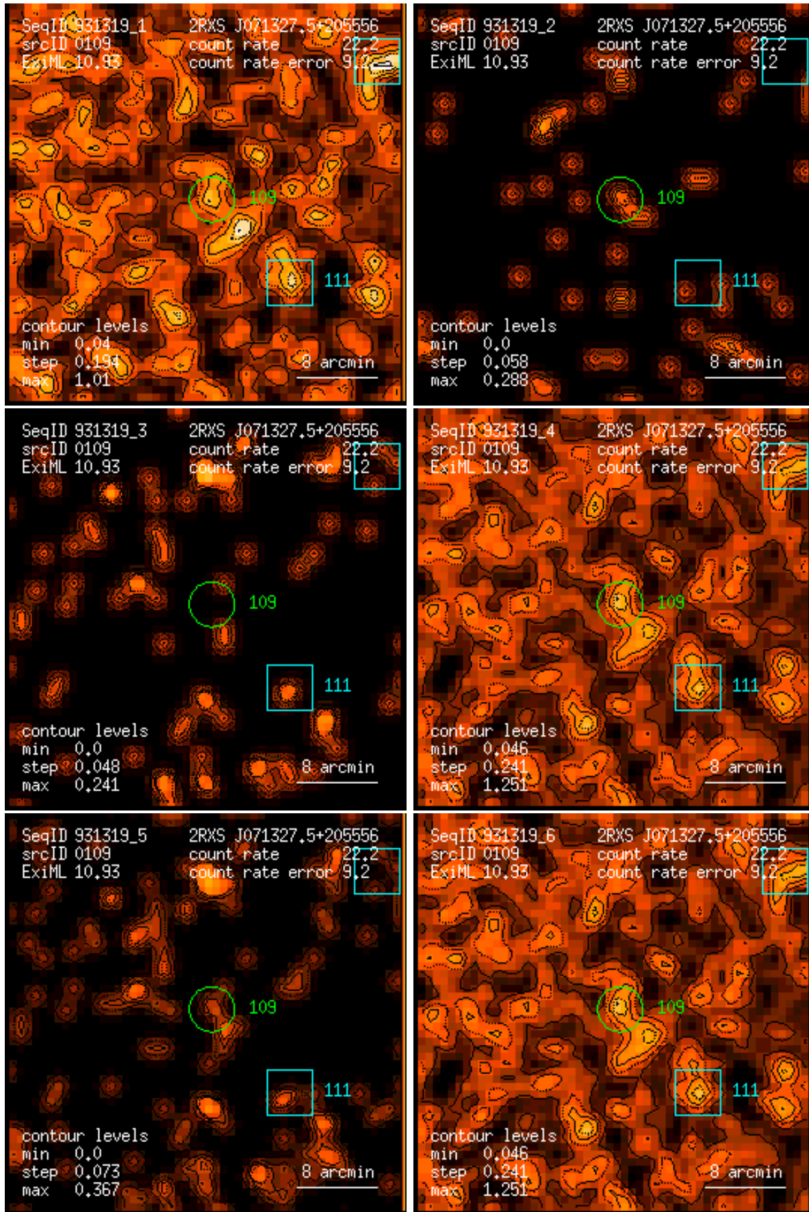
Figure 109: RASS 931319: detection 0109: band rate images, Gaussian filter: (1) PSPC channels 11 – 41, (2) 52 – 90, (3) 91 – 201, (4) 11 – 235, (5) 52 – 201, (6) 11 – 201. Broad band rates in counts/ks. Band rate contour levels in counts/ks/arcmin 2 .
