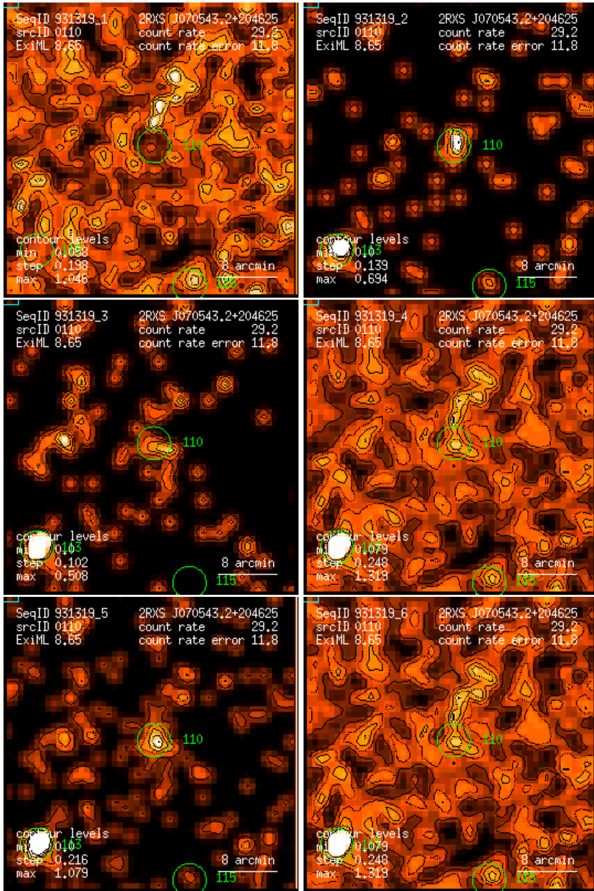
Figure 110: RASS 931319: detection 0110: band rate images, Gaussian filter: (1) PSPC channels 11 – 41, (2) 52 – 90, (3) 91 – 201, (4) 11 – 235, (5) 52 – 201, (6) 11 – 201. Broad band rates in counts/ks. Band rate contour levels in counts/ks/arcmin 2 .
