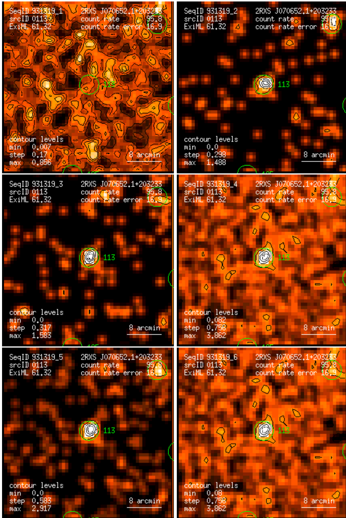
Figure 113: RASS 931319: detection 0113: band rate images, Gaussian filter: (1) PSPC channels 11 – 41, (2) 52 – 90, (3) 91 – 201, (4) 11 – 235, (5) 52 – 201, (6) 11 – 201. Broad band rates in counts/ks. Band rate contour levels in counts/ks/arcmin 2 .
