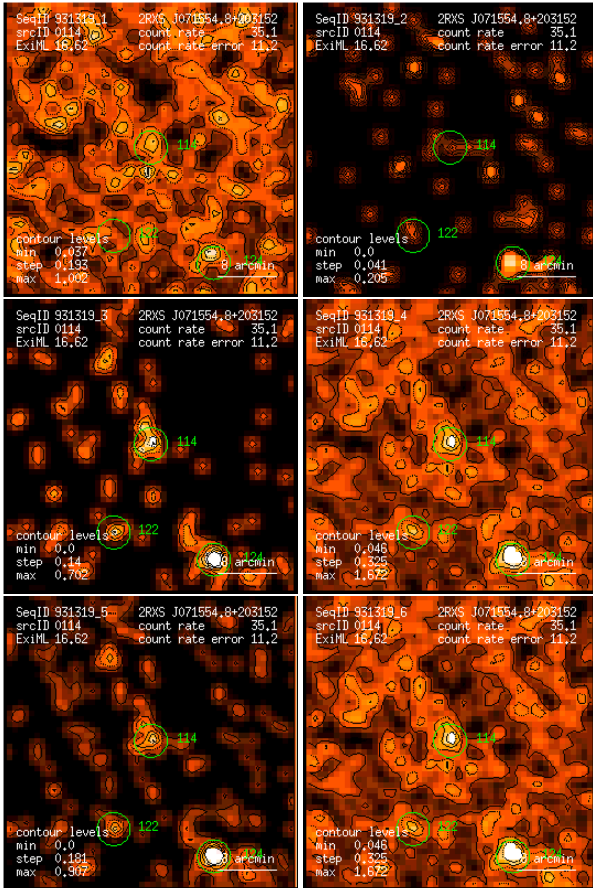
Figure 114: RASS 931319: detection 0114: band rate images, Gaussian filter: (1) PSPC channels 11 – 41, (2) 52 – 90, (3) 91 – 201, (4) 11 – 235, (5) 52 – 201, (6) 11 – 201. Broad band rates in counts/ks. Band rate contour levels in counts/ks/arcmin 2 .
