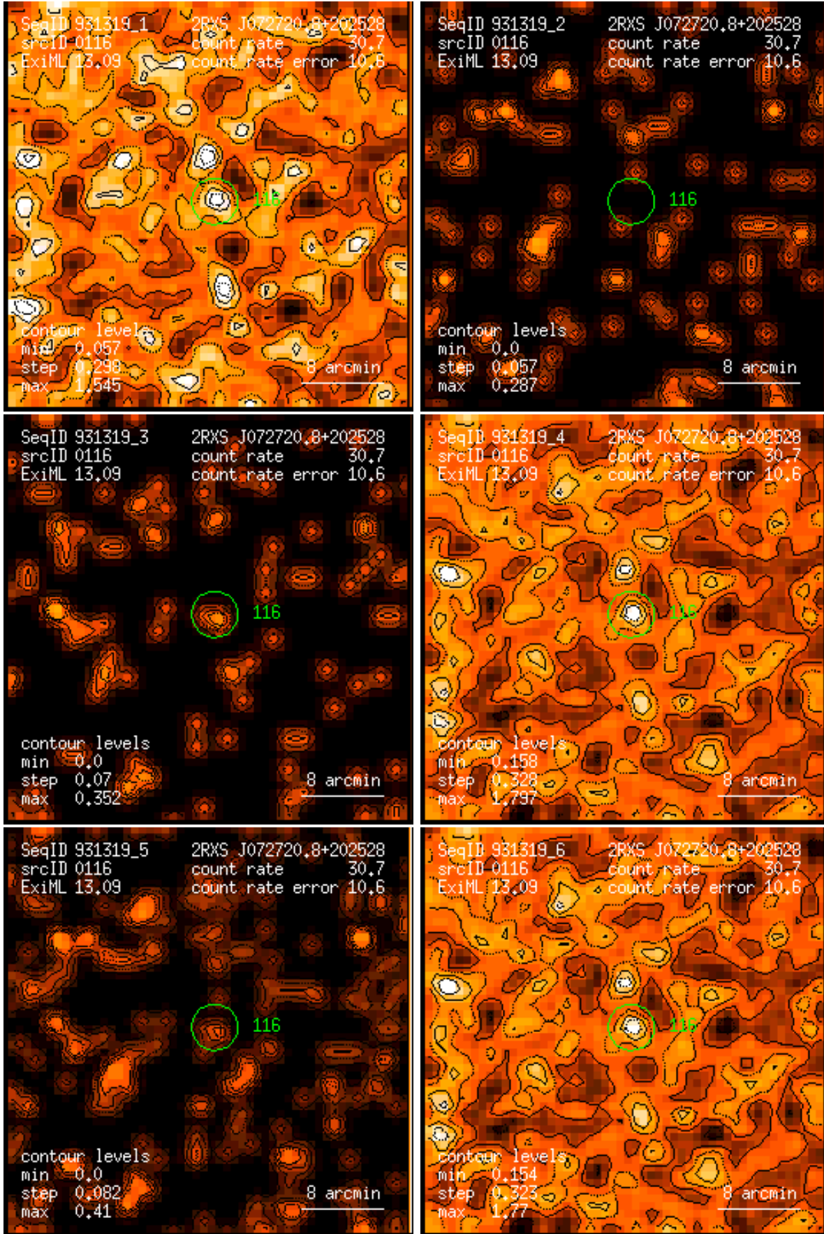
Figure 116: RASS 931319: detection 0116: band rate images, Gaussian filter: (1) PSPC channels 11 – 41, (2) 52 – 90, (3) 91 – 201, (4) 11 – 235, (5) 52 – 201, (6) 11 – 201. Broad band rates in counts/ks. Band rate contour levels in counts/ks/arcmin 2 .
