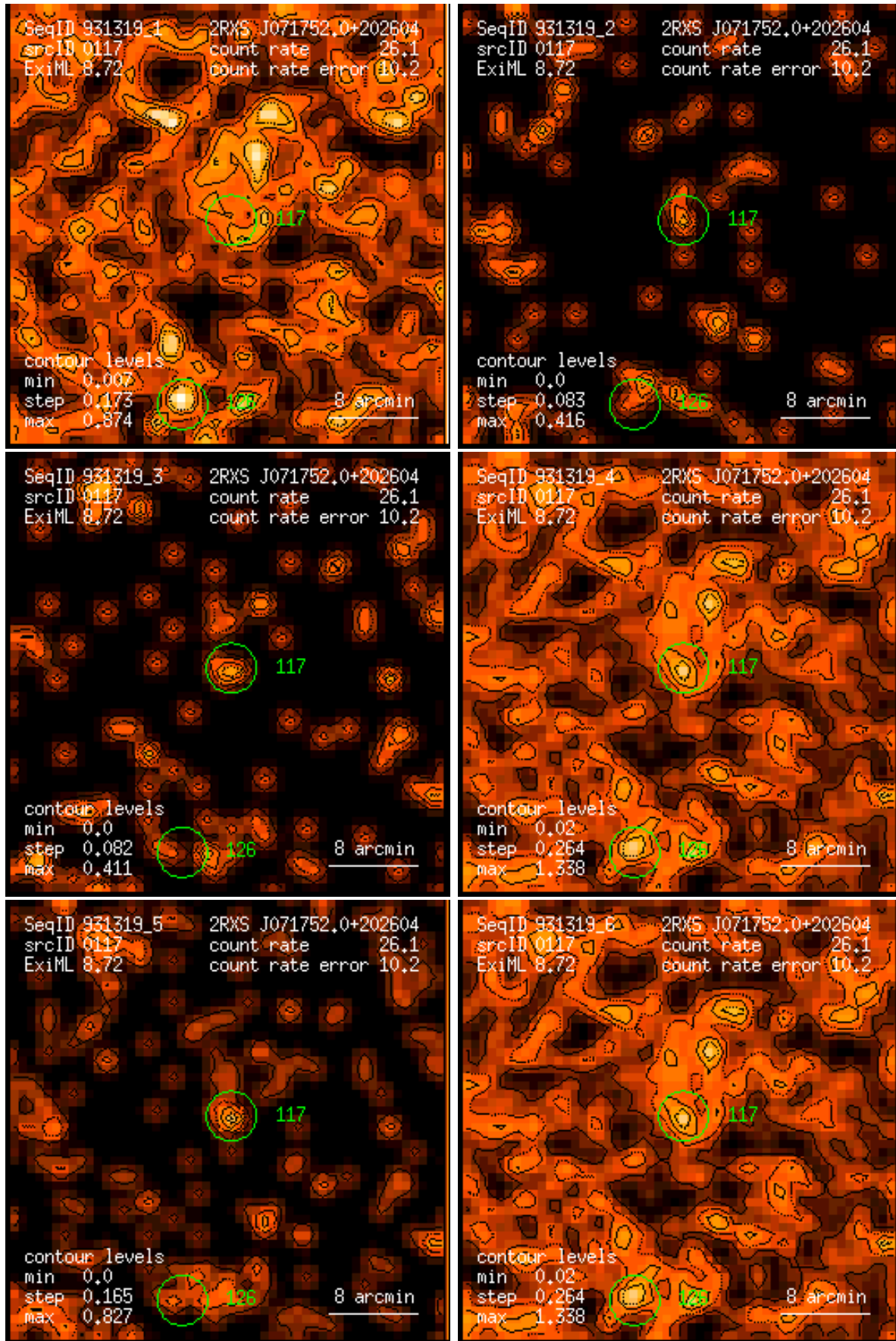
Figure 117: RASS 931319: detection 0117: band rate images, Gaussian filter: (1) PSPC channels 11 – 41, (2) 52 – 90, (3) 91 – 201, (4) 11 – 235, (5) 52 – 201, (6) 11 – 201. Broad band rates in counts/ks. Band rate contour levels in counts/ks/arcmin 2 .
