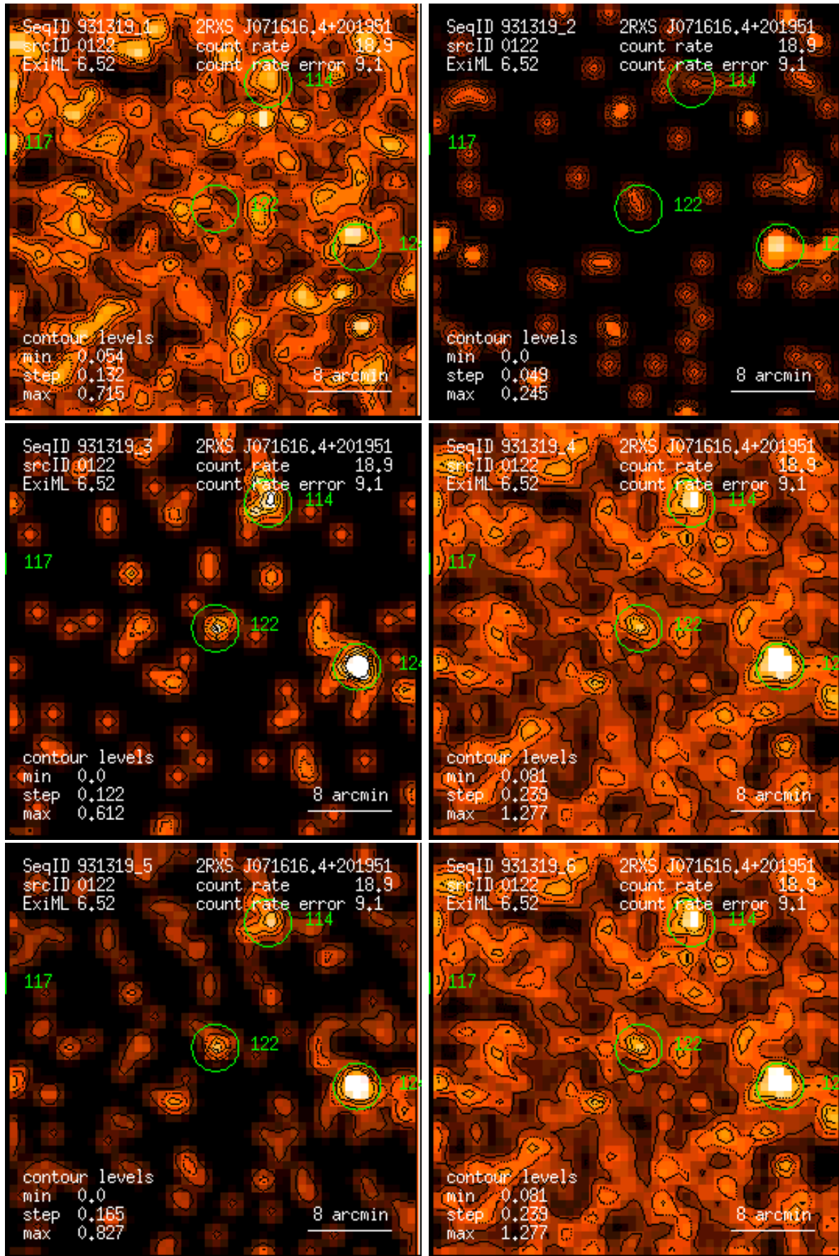
Figure 122: RASS 931319: detection 0122: band rate images, Gaussian filter: (1) PSPC channels 11 – 41, (2) 52 – 90, (3) 91 – 201, (4) 11 – 235, (5) 52 – 201, (6) 11 – 201. Broad band rates in counts/ks. Band rate contour levels in counts/ks/arcmin 2 .
