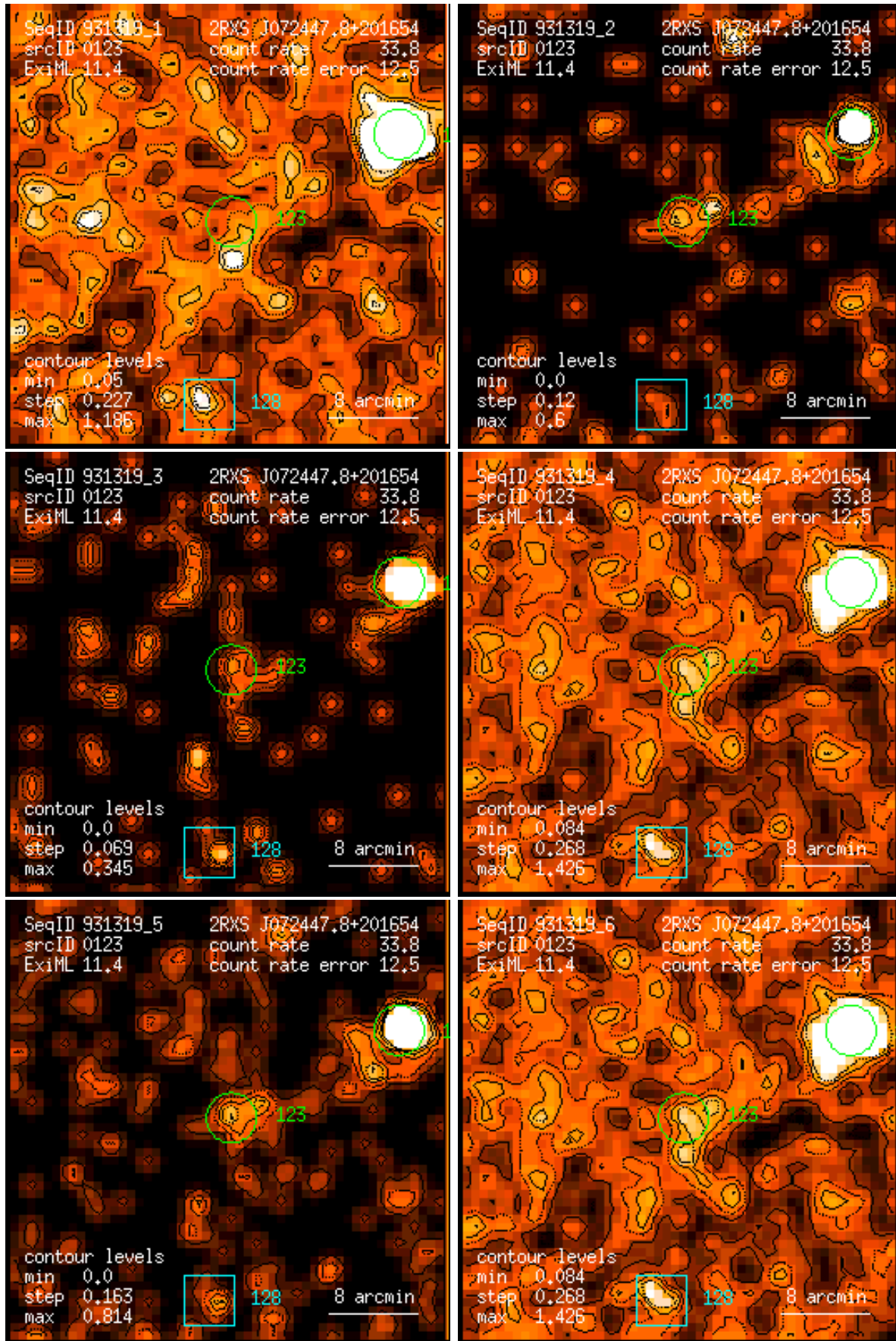
Figure 123: RASS 931319: detection 0123: band rate images, Gaussian filter: (1) PSPC channels 11 – 41, (2) 52 – 90, (3) 91 – 201, (4) 11 – 235, (5) 52 – 201, (6) 11 – 201. Broad band rates in counts/ks. Band rate contour levels in counts/ks/arcmin 2 .
