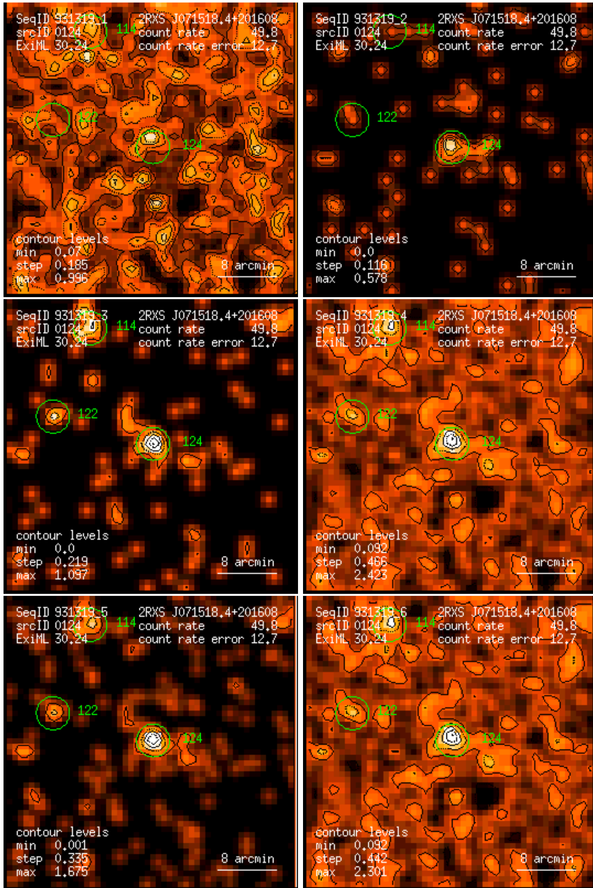
Figure 124: RASS 931319: detection 0124: band rate images, Gaussian filter: (1) PSPC channels 11 – 41, (2) 52 – 90, (3) 91 – 201, (4) 11 – 235, (5) 52 – 201, (6) 11 – 201. Broad band rates in counts/ks. Band rate contour levels in counts/ks/arcmin 2 .
