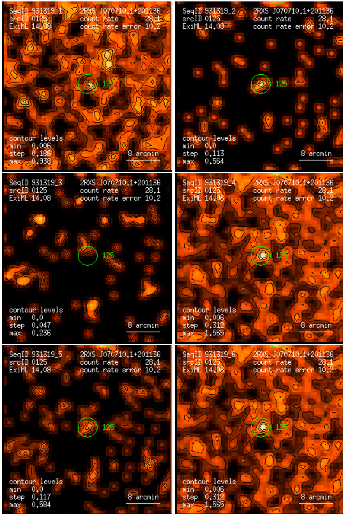
Figure 125: RASS 931319: detection 0125: band rate images, Gaussian filter: (1) PSPC channels 11 – 41, (2) 52 – 90, (3) 91 – 201, (4) 11 – 235, (5) 52 – 201, (6) 11 – 201. Broad band rates in counts/ks. Band rate contour levels in counts/ks/arcmin 2 .
