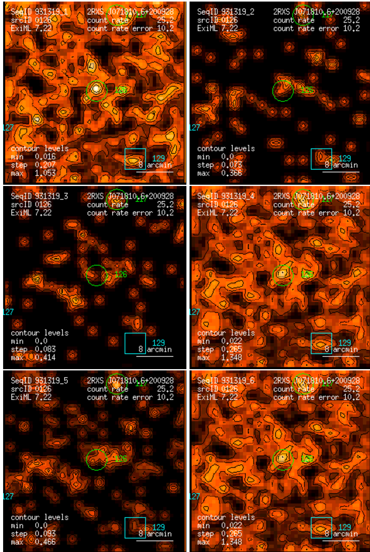
Figure 126: RASS 931319: detection 0126: band rate images, Gaussian filter: (1) PSPC channels 11 – 41, (2) 52 – 90, (3) 91 – 201, (4) 11 – 235, (5) 52 – 201, (6) 11 – 201. Broad band rates in counts/ks. Band rate contour levels in counts/ks/arcmin 2 .
