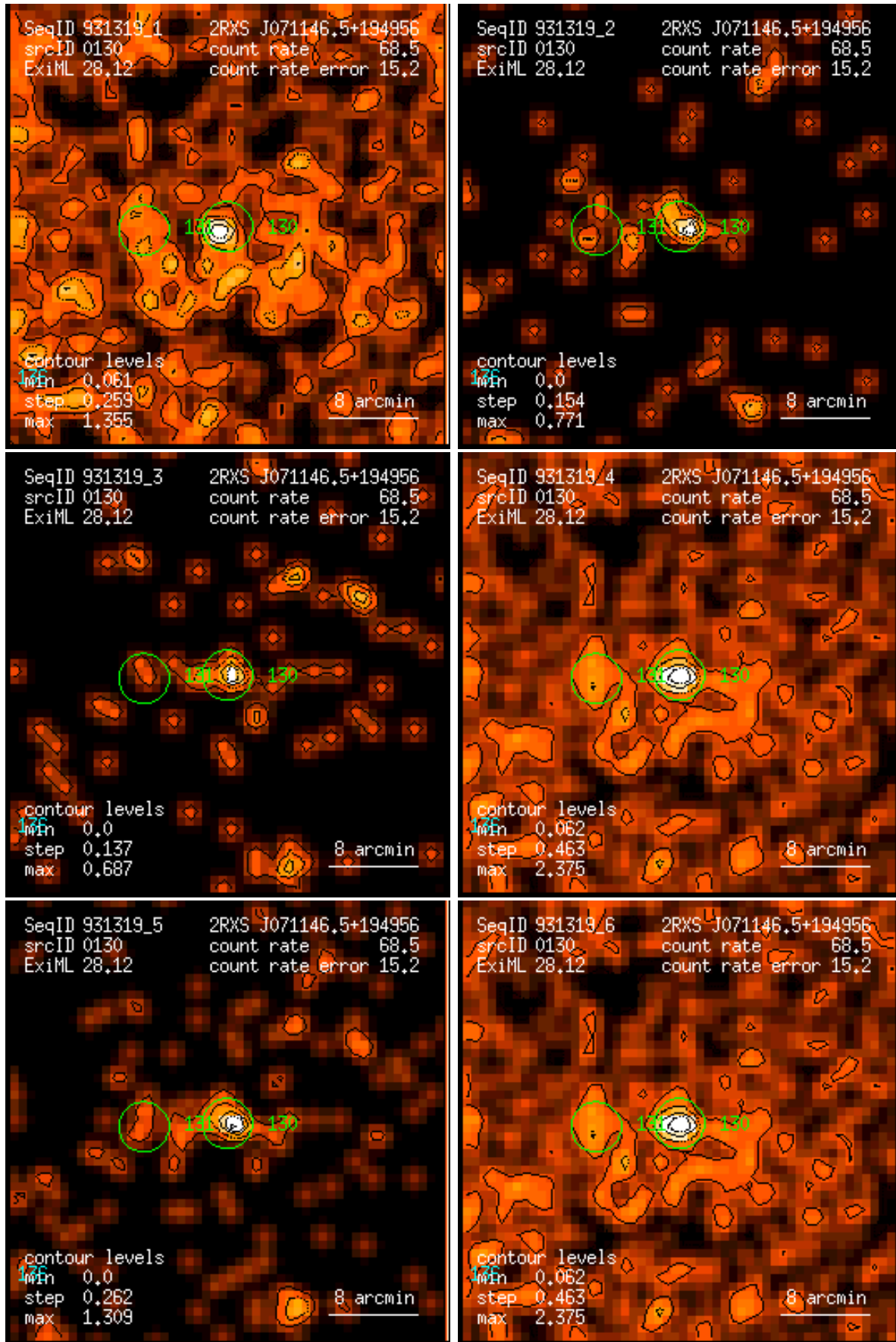
Figure 130: RASS 931319: detection 0130: band rate images, Gaussian filter: (1) PSPC channels 11 – 41, (2) 52 – 90, (3) 91 – 201, (4) 11 – 235, (5) 52 – 201, (6) 11 – 201. Broad band rates in counts/ks. Band rate contour levels in counts/ks/arcmin 2 .
