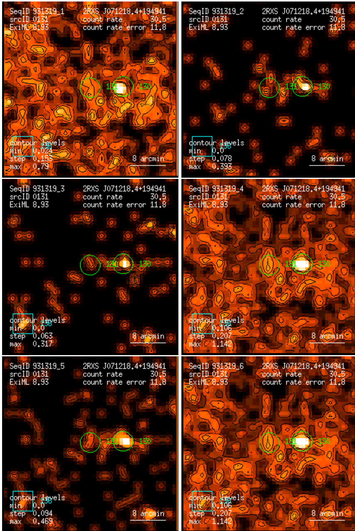
Figure 131: RASS 931319: detection 0131: band rate images, Gaussian filter: (1) PSPC channels 11 – 41, (2) 52 – 90, (3) 91 – 201, (4) 11 – 235, (5) 52 – 201, (6) 11 – 201. Broad band rates in counts/ks. Band rate contour levels in counts/ks/arcmin 2 .
