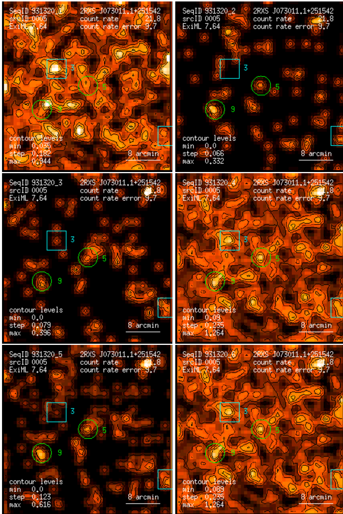
Figure 5: RASS 931320: detection 0005: band rate images, Gaussian filter: (1) PSPC channels 11 – 41, (2) 52 – 90, (3) 91 – 201, (4) 11 – 235, (5) 52 – 201, (6) 11 – 201. Broad band rates in counts/ks. Band rate contour levels in counts/ks/arcmin 2 .
