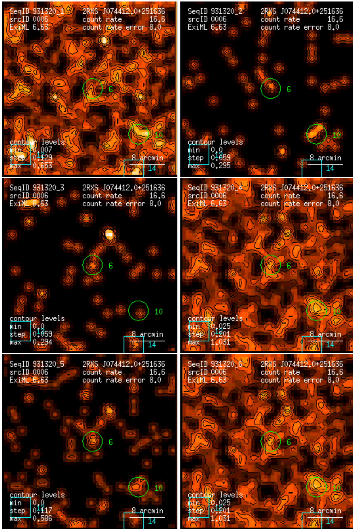
Figure 6: RASS 931320: detection 0006: band rate images, Gaussian filter: (1) PSPC channels 11 – 41, (2) 52 – 90, (3) 91 – 201, (4) 11 – 235, (5) 52 – 201, (6) 11 – 201. Broad band rates in counts/ks. Band rate contour levels in counts/ks/arcmin 2 .
