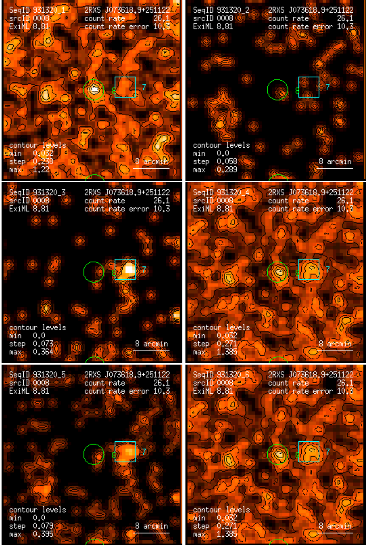
Figure 8: RASS 931320: detection 0008: band rate images, Gaussian filter: (1) PSPC channels 11 – 41, (2) 52 – 90, (3) 91 – 201, (4) 11 – 235, (5) 52 – 201, (6) 11 – 201. Broad band rates in counts/ks. Band rate contour levels in counts/ks/arcmin 2 .
