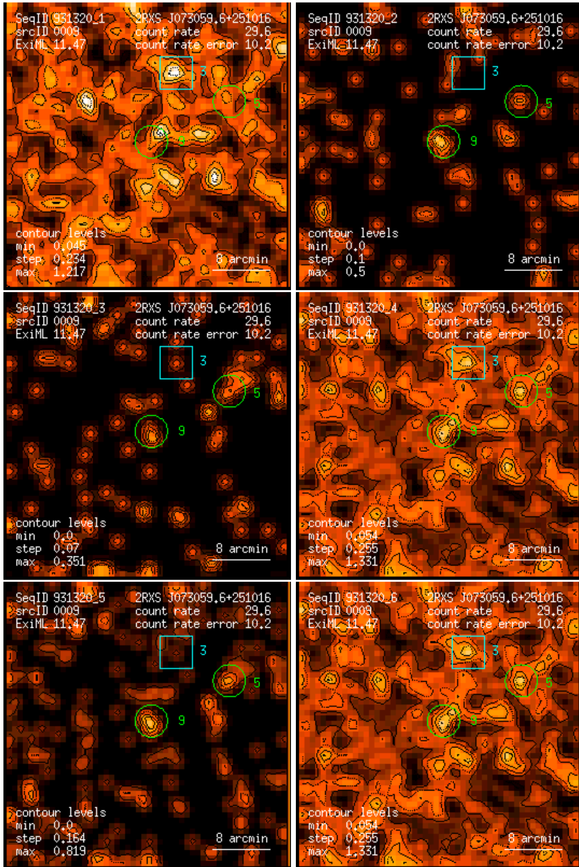
Figure 9: RASS 931320: detection 0009: band rate images, Gaussian filter: (1) PSPC channels 11 – 41, (2) 52 – 90, (3) 91 – 201, (4) 11 – 235, (5) 52 – 201, (6) 11 – 201. Broad band rates in counts/ks. Band rate contour levels in counts/ks/arcmin 2 .
